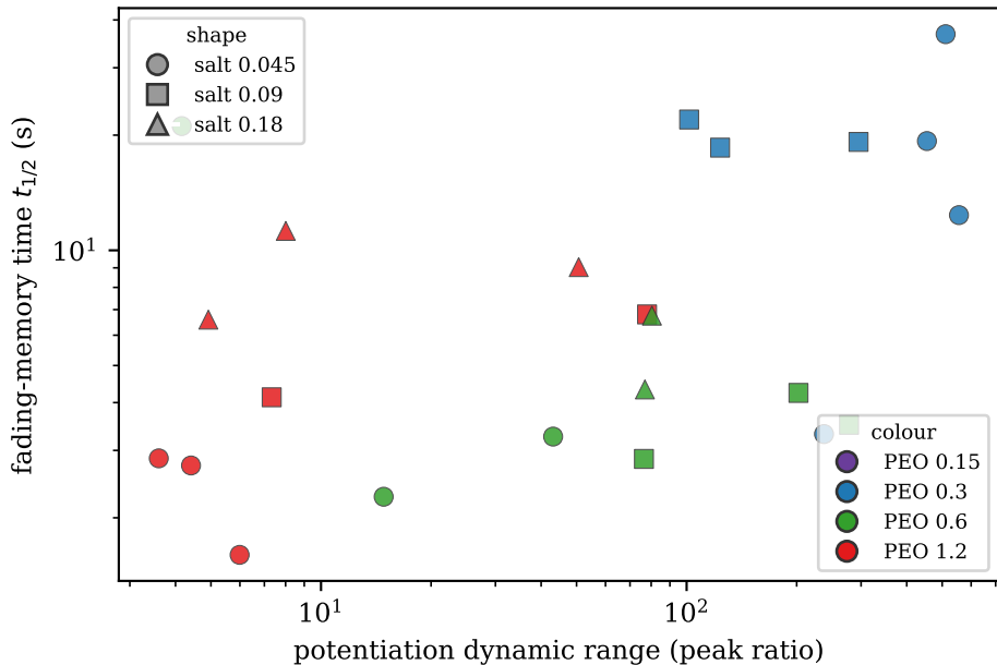
Per-device design space (Ag, Li)
