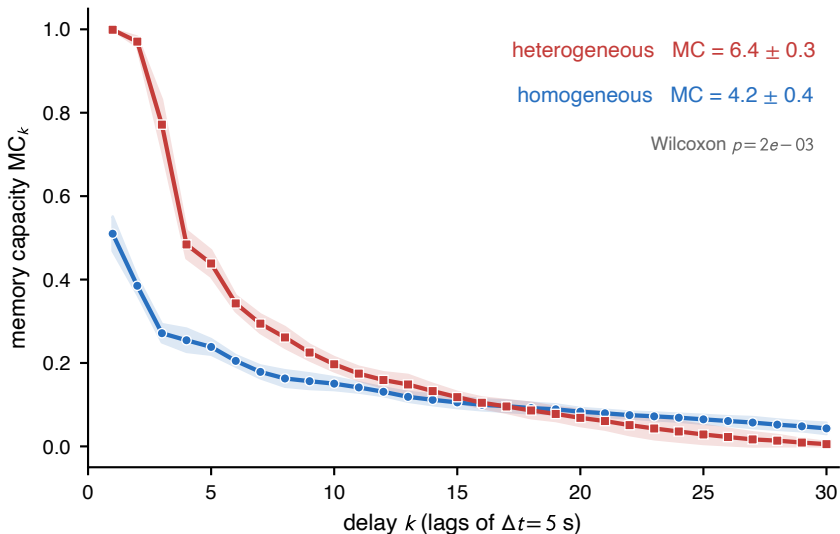
Memory capacity vs lag (N = 24 nodes)
