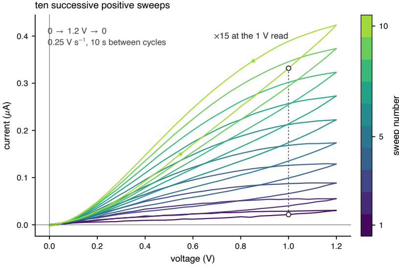
Figure 2.2: Current–voltage hysteresis of the composite memristive device. Ten successive positive triangular sweeps ( 0 \text{ V} \text{--} 1.2 \text{ V} , 0.25 \text{ V s}^{-1} , 10 s between cycles) fan out in near-uniform increments, the forward current at 1 V growing roughly 15-fold from the first to the tenth cycle. The clockwise loop closes at the origin (pinched hysteresis) without abrupt switching. Representative SY/Hybrane/LiOTf device (NM_v025) of the published 1:0.30:0.09 formulation, reproducing the hysteresis of Ref. [23].
