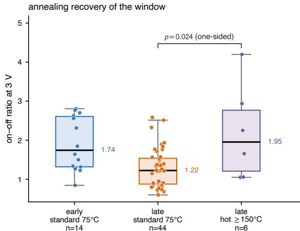
Figure 3.3: Annealing-recovery test of the hydrolysis hypothesis ( Hybrane /Ag, on-off ratio at \sim 3 V, per device). Among late devices, annealing at \geq 150 °C increases the median from 1.22 to 1.95, near the early-standard reference of 1.74; one-sided Mann–Whitney p = 0.024 . Interpretation is limited by n = 6 high-temperature devices, co-varying process changes, and pin issues in two devices. Reproduced by scripts/bridge_figures.py (F4).
