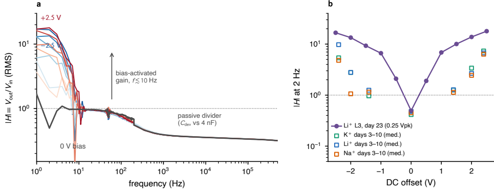
Figure 4.13: Frequency-domain face of the gold/TMPE/triflate devices (illustrative tier; Appendix C). (a) Transfer ratio |H|(f) of one \text{Li}^+ junction in series with 4 nF (day 23, 0.25 Vpk) at eleven DC offsets from 0 (grey) to \pm 2.5 V (blue negative, red positive): above \sim 1 kHz all curves collapse onto the passive capacitive divider; below \sim 10 Hz the bias activates a fundamental-frequency gain of up to \approx 18 , monotone in bias magnitude and near-symmetric in its sign. (b) Bias-gain curve: |H| at 2 Hz against DC offset for the day-23 series (line) and the per-cation medians of the earlier sessions (squares; days 3–10, 0.4 Vpk–1.4 Vpk); gain requires bias, grows with it, and appears for all three cations.
