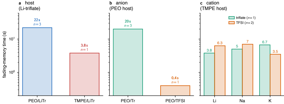
Figure 4.7: Illustrative effect of electrolyte chemistry on the fading-memory time constant ( Super Yellow , 0.3/0.09, silver, matched 4V/2V protocol). Host (PEO vs TMPE, Li-triflate) and anion (triflate vs TFSI, PEO host) produce the largest shifts. The cation panel shows the same three cations in the TMPE host under each anion: the order inverts with the anion (potassium longest in triflate, shortest in TFSI), so the cation produces no consistent, host- and anion-independent ordering. Sample sizes are small ( n as labelled); see text.
