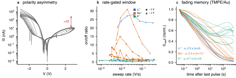
Figure 4.12: The negative-polarity face of the gold/TMPE/triflate devices (illustrative tier; Appendix C). (a) Exemplar bipolar sweep ( \pm 3 V, ten cycles, \text{Na}^+ device): the negative branch carries \approx 42\times the current of the positive one. (b) The switching window is rate-gated: on–off ratio against sweep rate for all step-count series (colour = cation, marker = amplitude); slow sweeps open windows of 20–31 where the standard fast protocol reads \approx 1 . (c) Fading memory of the TMPE host on gold: sparse-read relaxations after -5 V pulse trains, normalised to the first read, with per-cation median half-decay times, seconds-scale, as on silver, and far below PEO on gold.
