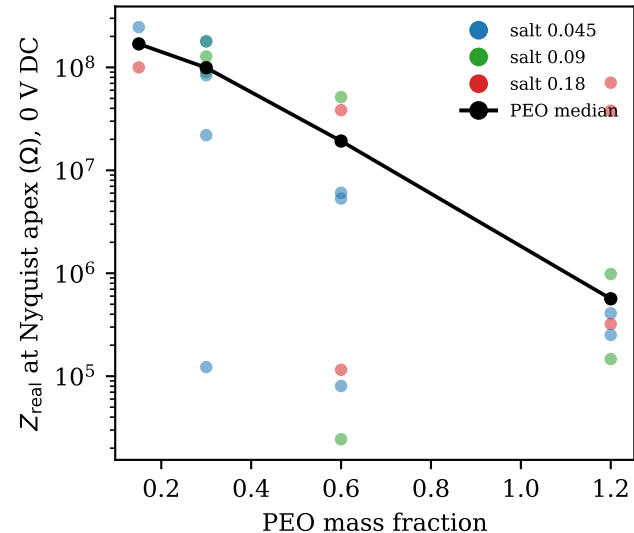
(a) Ionic impedance vs composition
