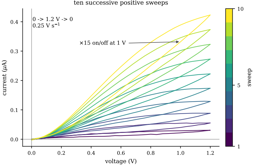
Figure 2.2: Current–voltage hysteresis of the composite memristive device. Ten successive positive triangular sweeps ( 0\text{ V} – 1.2\text{ V} , 0.25\text{ V s}^{-1} , 10\text{ s} between cycles) fan out in near-uniform increments, the forward current at 1\text{ V} growing roughly 15-fold from the first to the tenth cycle. The clockwise loop closes at the origin (pinched hysteresis) without abrupt switching. Representative SY/Hybrane/LiOTf device (NM_v025) of the published 1:0.30:0.09 formulation, reproducing the hysteresis of Ref. [27].
