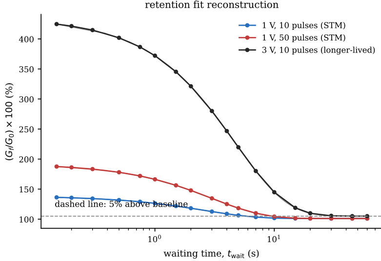
Figure 2.4: Memory retention kinetics. Conductance ratio (G_f/G_0) \times 100\% versus waiting time t_{\text{wait}} for STM conditions (1 V; 10 and 50 pulses, blue/red) and the longer-lived regime denoted LTM (3 V, 10 pulses, black). Solid lines are standard-exponential reconstructions of the form in ??; the fit parameters are summarised in Appendix A. Data and fit parameters from Ref. [27].
