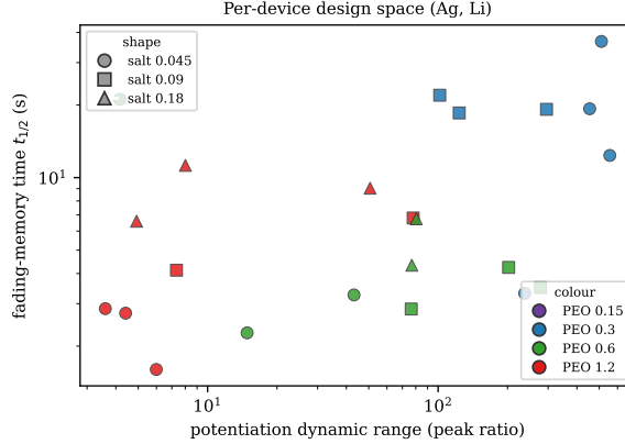
Figure 3.8: Per-device design space of the Super Yellow /PEO/LiOTf/Ag composition grid: fading-memory time t_{1/2} against potentiation dynamic range (peak ratio), coloured by PEO fraction and marked by salt fraction (one point per device, median over its pixels). The PEO fraction selects the broad region a device occupies — low PEO (blue) in the long-memory, high-dynamic-range corner, high PEO (red) in the opposite one, so memory and nonlinearity are not independently tunable but paired . The substantial within-composition scatter is the genuine device-to-device heterogeneity that Chapter 4 exploits; it is shown, not averaged away.
