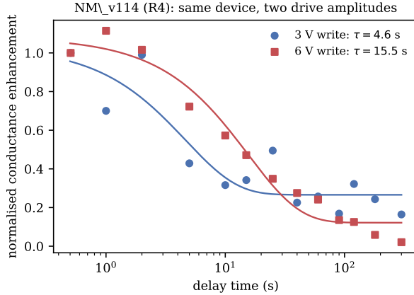
Figure 3.6: The apparent fading-memory time is set in part by the drive protocol. The same device, measured under a larger write/read amplitude, shows a markedly longer apparent relaxation time.
