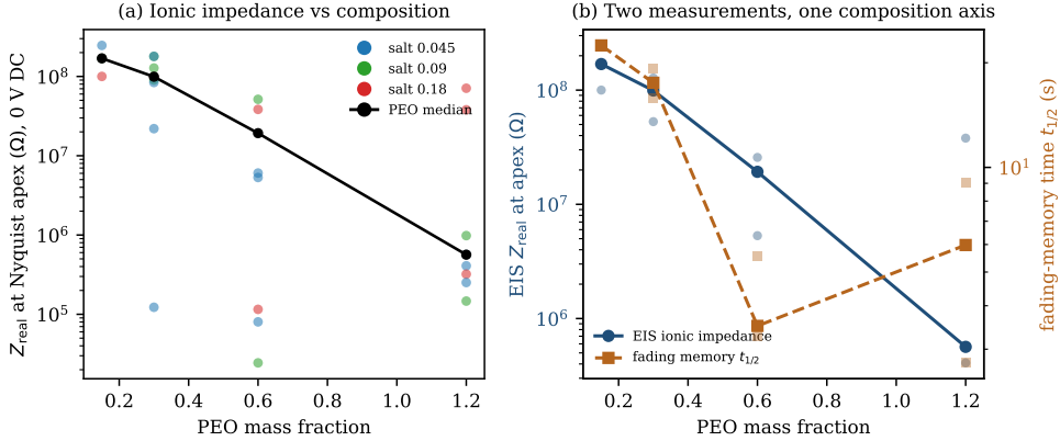
Figure 3.7: Equilibrium (0 V-DC) impedance spectroscopy corroborates the composition control of the dynamics (silver Super Yellow /PEO/LiOTf grid). (a) The impedance resistance scale — here the model-free real impedance at the Nyquist apex — falls by more than three orders of magnitude as the PEO fraction rises (points are devices, coloured by salt; the black line is the PEO median). (b) The equilibrium impedance scale (left axis) and the independently measured fading-memory time t_{1/2} (right axis) decline along the same PEO composition axis (cell-level points with per-PEO median trends): the two are co-driven by composition, not independent knobs. Analysis in scripts/ch3_eis.py ; per-cell values in handouts/ch3_eis_by_cell.csv .
