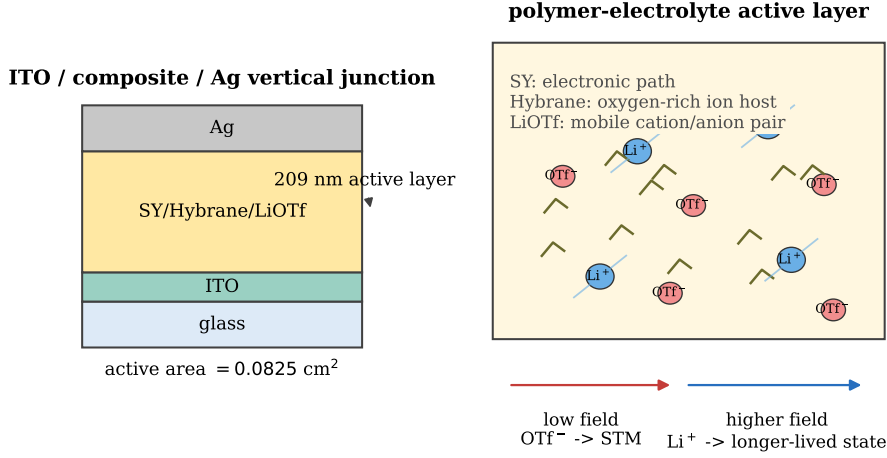
Figure 2.1: Schematic of the two-terminal vertical synaptic device and active-layer mechanism. The device stack is ITO-glass / Super Yellow /Hybrane/LiOTf composite / Ag; the composite separates the electronic pathway, ion-transport host, and mobile-ion supply. The proposed mechanism assigns the faster STM response to weakly coordinated triflate redistribution and the longer-lived state to displacement of strongly coordinated Li + . Schematic generated from the device geometry and mechanism reported in Ref. [23].
