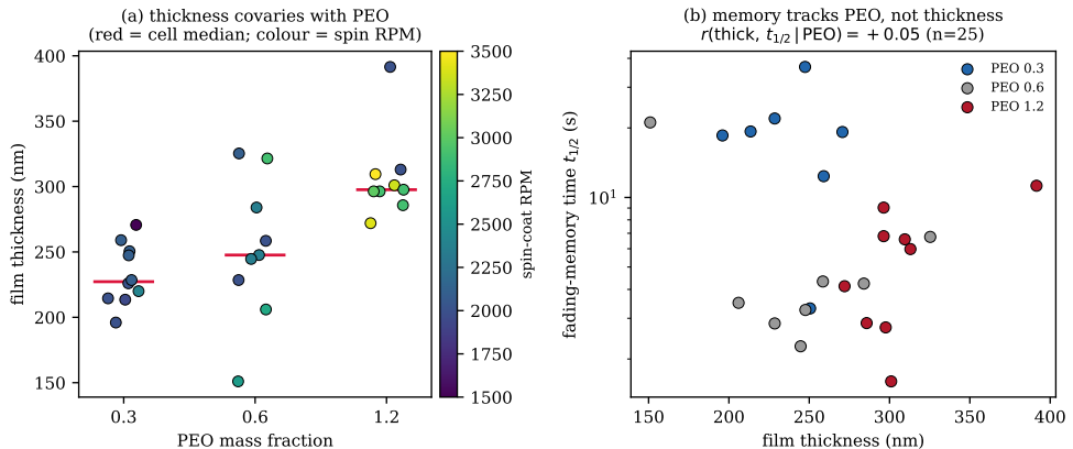
Figure 4.1: Film thickness covaries with composition but does not drive the dynamics (silver composition spine, n = 30 ). (a) Film thickness rises with PEO fraction (red bars are cell medians); the spin-coating speed (colour) was raised for higher-PEO cells to partially equalise thickness, but the compensation is incomplete. (b) The fading-memory time t_{1/2} is set by composition (PEO colour), not by thickness (horizontal axis): within each PEO band the timescale is flat against thickness, and the partial correlation of thickness with t_{1/2} controlling for PEO is \approx 0 . Data from DEVICES_PROFILOMETRY_STATS.csv ; see handouts/14_thickness_rpm_confound_audit.md .
