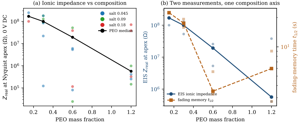
Figure 4.10: Equilibrium (0 V-DC) impedance spectroscopy corroborates the composition control of the dynamics (silver Super Yellow /PEO/LiOTf grid). (a) The impedance resistance scale — here the model-free real impedance at the Nyquist apex — falls by more than three orders of magnitude as the PEO fraction rises (points are devices, coloured by salt; the black line is the PEO median). (b) The equilibrium impedance scale (left axis) and the independently measured fading-memory time t_{1/2} (right axis) decline along the same PEO composition axis (cell-level points with per-PEO median trends): the two are co-driven by composition, not independent knobs. Analysis in scripts/ch3_eis.py ; per-cell values in handouts/ch3_eis_by_cell.csv .
