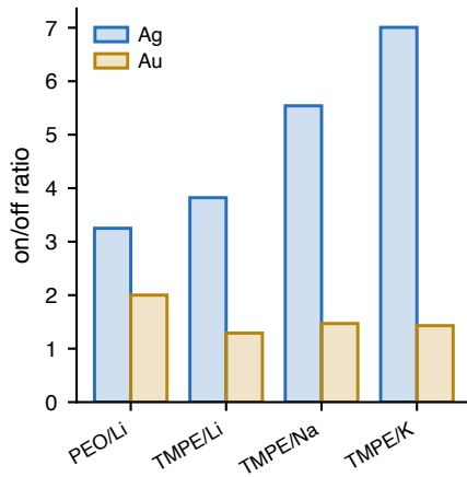
b switching window
