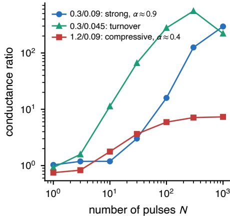
b pulse potentiation
