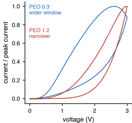
a hysteresis loop (norm., salt 0.09)
