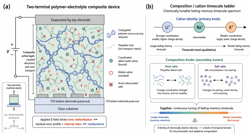
Figure 1.14: The thesis-specific polymer-electrolyte composite device and its chemically tunable dynamical timescale. (a) Vertical two-terminal stack: a solution-processed composite active layer combines a conjugated semiconducting polymer network with an oxygen-rich ion-conducting host and alkali-metal salt, between a patterned ITO bottom electrode and an evaporated silver top electrode; the working model assigns memory to a residual ionic distribution after bias. (b) Timescale ladder as anticipated at the design stage , with cation identity drawn as the primary control and the host-to-semiconductor and salt-to-semiconductor mass ratios as secondary ones, placing the fading-memory time along the \text{Li}^+ > \text{Na}^+ > \text{K}^+ coordination order. The panel records the starting hypothesis, not the result. Chapter 4 inverts this hierarchy: composition (the PEO/SY and salt/SY mass ratios) is the replicated quantitative control of the timescale, whereas the cation is sample-limited and its anticipated ordering is not borne out (the triflate retention series runs in reverse).
