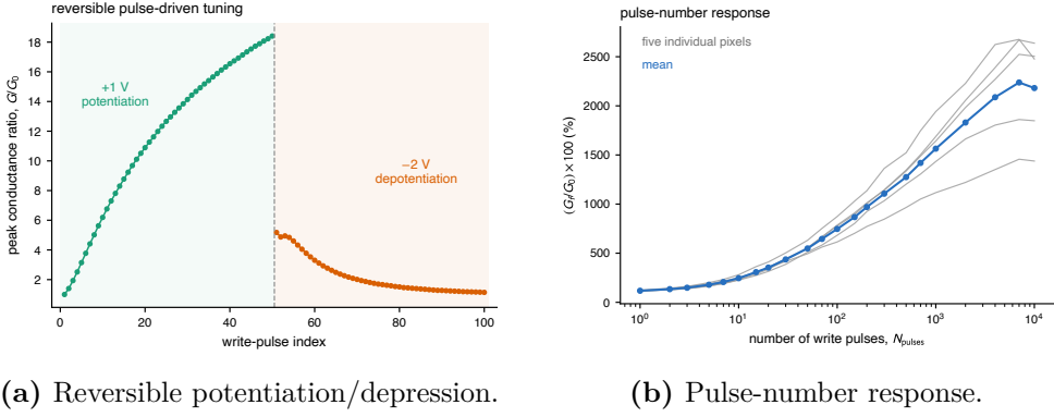
Figure 2.3: Pulse-driven conductance integration in the composite memristive platform. (a) Fifty consecutive 1 V write pulses continuously potentiate junction L5 on NM_v055; subsequent -2 \text{ V} pulses depotentiate it toward the initial state. (b) Dependence of the conductance ratio (G_f/G_0) \times 100\% on the number of write pulses for V_{\text{write}} = 1 \text{ V} and t_{\text{wait}} = 150 \text{ ms} . Thin grey lines are five crossbar junctions on the same NM_v055 substrate; the bold line is their mean. The spread therefore measures within-substrate junction variability, not device- or batch-level reproducibility. Data regenerated from the local archive associated with Ref. [22].
