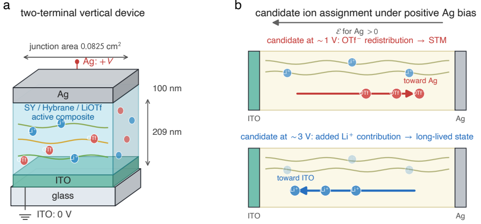
Figure 2.1: Schematic of the two-terminal vertical synaptic device and candidate active-layer mechanism. The device stack is ITO-glass / Super Yellow / Hybrane / LiOTf composite / Ag; the composite separates the electronic pathway, ion-transport host, and mobile-ion supply. The species labels show the working fast-anion/slow-cation assignment reported in Ref. [22], not a direct measurement of ion motion; the comparative cation data do not establish that assignment as a general law.
