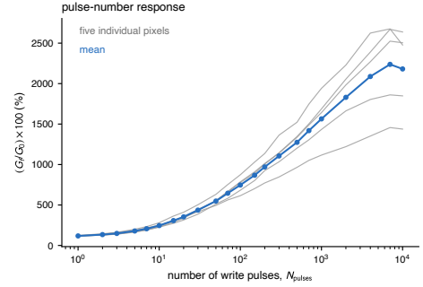
(b) Pulse-number response.
