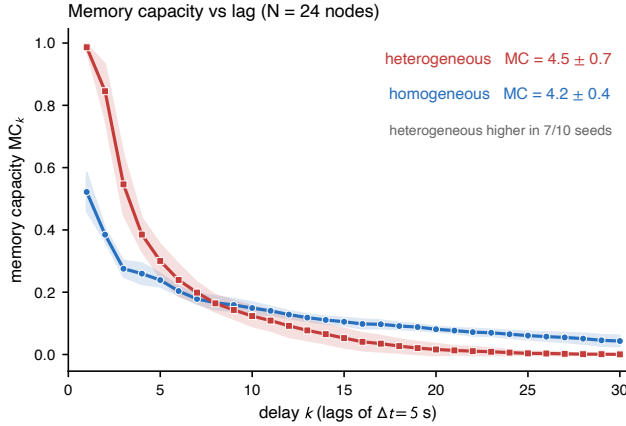
Figure 5.1: Linear memory capacity MC_k as a function of delay k for a homogeneous bank (all PEO 0.3/0.09 nodes) versus a heterogeneous composition bank ( \tau \approx 4\text{--}30\text{ s} ). Under the bounded, peak-calibrated node model, total capacity is 4.19 \pm 0.42 and 4.52 \pm 0.67 , respectively; the heterogeneous value is higher in seven of ten seed pairs. Its main effect is a redistribution toward the shortest lags, not a resolved increase in total linear capacity. Shaded bands are \pm 1 SD over ten random input/bank seeds. Seeds quantify algorithmic sensitivity rather than experimental replication. N = 24 independent leaky nodes, random uniform input, linear ridge read-out.
