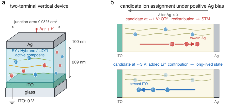
Figure 2.1: Schematic of the two-terminal vertical synaptic device and candidate active-layer mechanism. The device stack is ITO-glass / Super Yellow /Hybrane/LiOTf composite / Ag; the composite separates the electronic pathway, ion-transport host, and mobile-ion supply. The species labels show the working fast-anion/slow-cation assignment reported in Ref. [6], not a direct measurement of ion motion; the comparative cation data do not establish that assignment as a general law.
