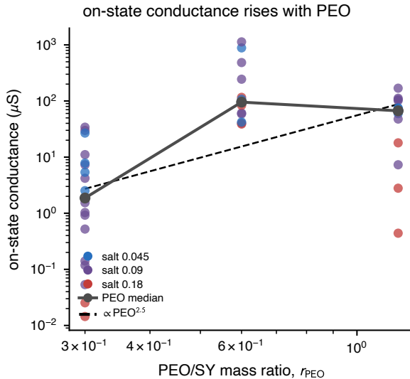
Figure C.2: Absolute on-state conductance (HYST, conductance at the sweep maximum; substrate medians from the replicated Ag series, coloured by r_{\text{salt}} ) against r_{\text{PEO}} , log–log. The positive overall association (statistics printed in the panel) has the opposite sign to simple electronic-percolation dilution. Cell medians are not strictly monotone, and the raised-floor account in section 4.9 remains a candidate mechanism.
