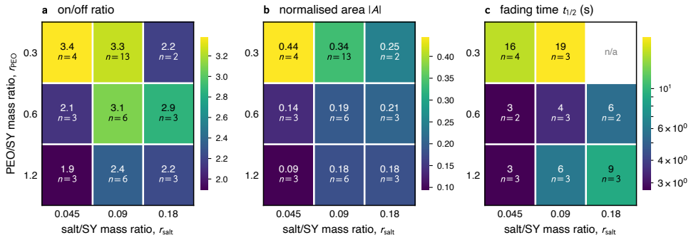
Figure 4.3: Composition control of the steady-state and dynamical response of Super Yellow /PEO/LiOTf devices. The switching window (a, b) and the fading-memory time (c) both decrease as the PEO-to- Super Yellow mass ratio increases at fixed salt ratio.
