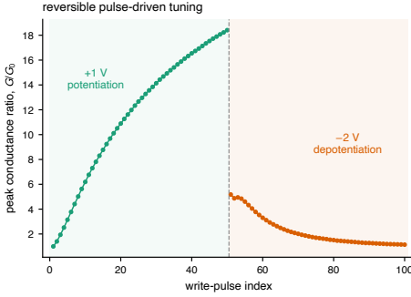
(a) Reversible potentiation/depression.
