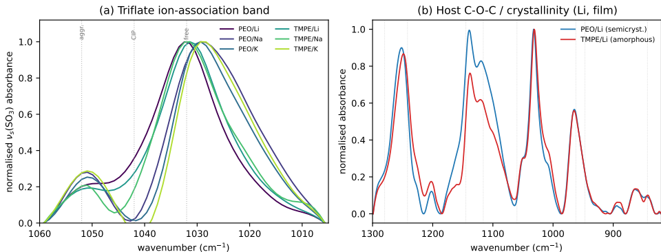
Figure 3.4: ATR-FTIR corroboration of the chemistry axis (electrode-free Super Yellow -blend films/powders, 0.3/0.09, one specimen per chemistry). (a) The triflate ion-association band \nu_s(\text{SO}_3) , whose position reports the ion-association state (spectroscopically free near 1032 cm -1 , contact ion pair near 1042 cm -1 , aggregate above; reference positions dotted), sits at 1029 cm -1 –1032 cm -1 in every host \times cation sample with no cation-resolved shift — microscopically consistent with the cation not being a clean retention lever. (b) The polyether C–O–C / crystallinity envelope of the linear PEO host (blue) is a resolved multiplet (semicrystalline), whereas the hyperbranched TMPE host (red) collapses it into a single broad, amorphous band. Spectra are normalised after a local/rubber-band baseline; intensities are not comparable across specimens (mixed film/powder sampling), so only band positions and shapes are read. Analysis in scripts/ch3_iratr.py ; full assessment in handouts/16_iratr_assessment.md .
