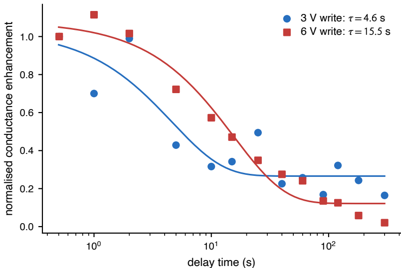
device NM_v114 (R4): same device, two drive amplitudes
