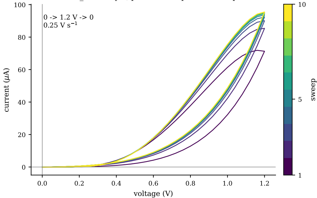
NM_v055 Day 1, pixel L4: ten positive sweeps
