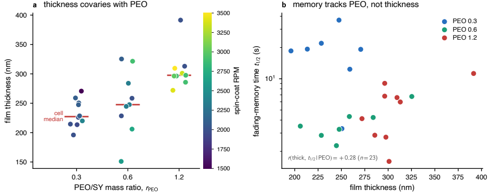
Figure 4.1: Film thickness and fading-memory time in the replicated silver composition grid. (a) Film thickness rises with r_{PEO} (red bars are cell medians; n = 28 substrates with profilometry and a dynamical measurement); higher-PEO cells were spun faster (colour) to reduce this difference, although residual covariation remains. (b) For the n = 23 substrates with t_{1/2} , the partial correlations are r_{\text{partial}}(\text{thickness}, \log t_{1/2} | r_{PEO}) = +0.28 and r_{\text{partial}}(r_{PEO}, \log t_{1/2} | \text{thickness}) = -0.51 . Thickness does not remove the composition association, but a secondary thickness contribution is not excluded.
