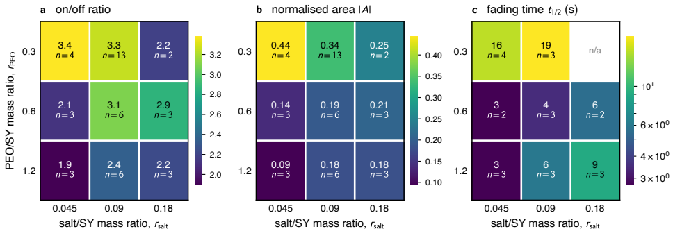
Figure 4.3: Composition control of the steady-state and dynamical response of Super Yellow /PEO/LiOTf devices. Across the replicated grid, increasing the PEO-to- Super Yellow mass ratio is associated overall with smaller switching windows (a, b) and shorter fading-memory times (c). Individual fixed-salt rows are not strictly monotone, especially in the sparsely sampled salt-rich cells.
