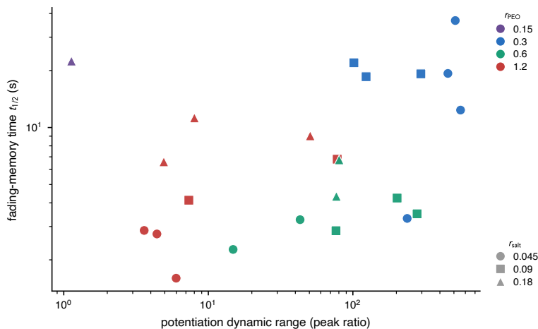
Figure 4.14: Per-substrate design space of the Super Yellow /PEO/LiOTf/Ag composition grid: fading-memory time t_{1/2} against potentiation dynamic range (peak ratio), coloured by r_{PEO} and marked by r_{salt} (one point per fabricated substrate, median over its junctions). The PEO ratio selects the broad region a substrate occupies: low PEO (blue) in the long-memory, high-dynamic-range corner, high PEO (red) in the opposite one, so memory and nonlinearity are paired , not independently tunable. The substantial within-composition scatter is the genuine substrate-to-substrate heterogeneity that Chapter 5 exploits.
