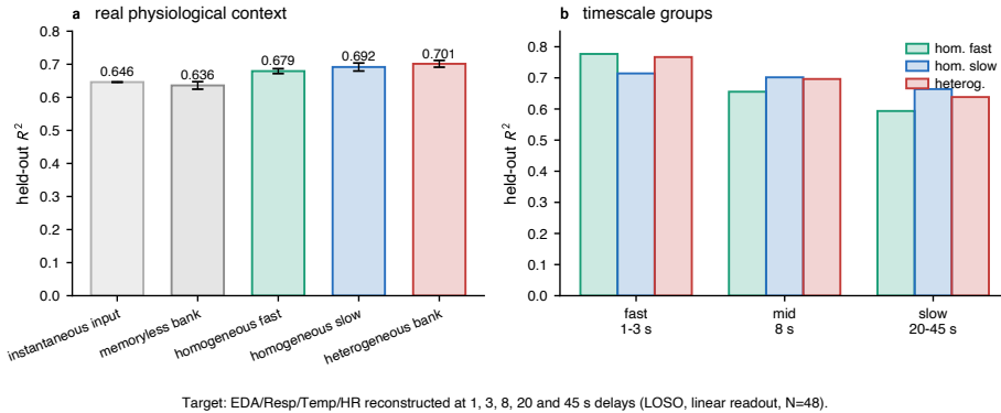
Figure 5.5: Multi-lag physiological context reconstruction on real WESAD streams (chest EDA, respiration, temperature, and causally derived heart rate). A linear read-out reconstructs each channel at delays of 1, 3, 8, 20 and 45 s (leave-one-subject-out, N = 48 ). The heterogeneous bank gives the highest overall subject-mean R^2 (0.701), ahead of the slow homogeneous control (0.692) and instantaneous input (0.646). The zero-based axes avoid magnifying these modest differences.
