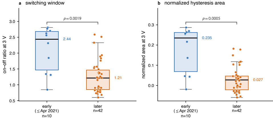
Figure 3.1: Switching-window reduction across the campaign on the standard Super Yellow/Hybrane/LiOTf/Ag corpus, read at the \sim 3 V stratum where the window is expressed, one value per device. (a) On-off ratio and (b) normalized hysteresis area, both for devices fabricated before the NM_v026 change point ( \leq Apr 2021) versus later. Boxes are quartiles with the median annotated beside each box; points are individual devices; the bracket gives the two-sided Mann-Whitney p . The on-off ratio decreases by roughly a factor of two and the area by an order of magnitude. Reproduced by scripts/bridge_figures.py (F1).
