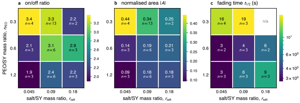
Figure 4.3: Composition control of the steady-state and dynamical response of Super Yellow /PEO/LiOTf devices. Across the replicated grid, increasing the PEO-to- Super Yellow mass ratio is associated overall with smaller switching windows (a, b) and shorter fading-memory times (c). Individual fixed-salt rows are not strictly monotone, especially in the sparsely sampled salt-rich cells.
