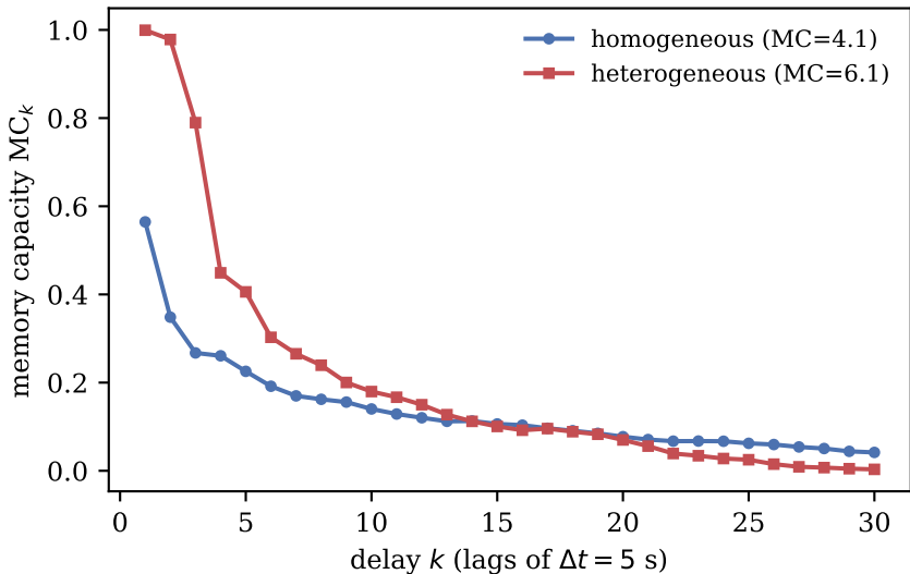
Memory capacity vs lag (N=24 nodes)
