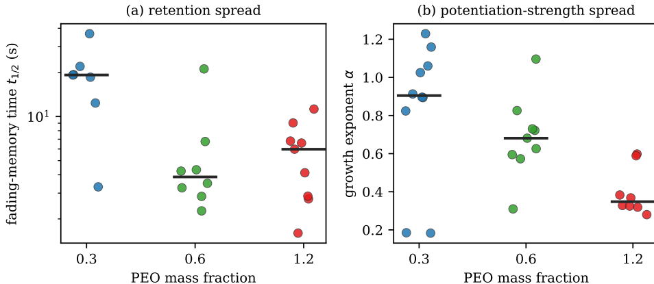
Figure 3.4: The cell medians of fig. 3.3 are summaries of genuinely spread distributions, not tight clusters (one point per device, Super Yellow /PEO/LiOTf/Ag; black bar is the cell median). (a) Fading-memory time t_{1/2} and (b) potentiation growth exponent \alpha , each against PEO fraction. The PEO fraction sets the broad level, but within every composition cell the device-to-device variation is comparable to the steps between cells — the heterogeneity that Chapter 4 treats as a resource rather than averaging away. Shown, not averaged; from handouts/ch4_decay_fits.csv and ch4_pulse_descriptors.csv .
