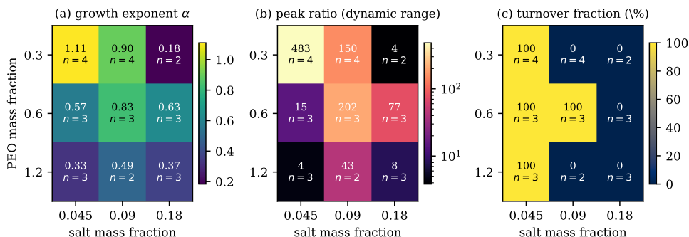
Figure 3.5: Potentiation (pulse-integration) response across the Super Yellow /PEO/LiOTf composition grid: (a) the log–log growth exponent \alpha , (b) the peak conductance ratio (usable dynamic range, log scale), and (c) the fraction of devices whose response turns over within the measured range ( N \leq 1000 ). Increasing the PEO fraction lowers \alpha and the dynamic range; increasing the salt fraction suppresses turnover, sustaining growth to higher pulse counts. Per-cell median, with the device count n annotated in each cell.
