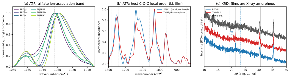
Figure 3.6: Microscopic corroboration of the chemistry axis (electrode-free Super Yellow -blend films/powders, 0.3/0.09, one specimen per chemistry). (a) ATR-FTIR triflate ion-association band \nu_s(\text{SO}_3) , whose position reports the ion-association state (spectroscopically free near 1032\text{ cm}^{-1} , contact ion pair near 1042\text{ cm}^{-1} , aggregate above; reference positions dotted [2]): it sits at 1029\text{ cm}^{-1} – 1032\text{ cm}^{-1} in every host \times cation sample with no cation-resolved shift — microscopically consistent with the cation not being a clean retention lever. (b) ATR-FTIR C–O–C envelope: the linear PEO host (blue) shows a resolved multiplet, i.e. retained local (conformational) ether-backbone order, whereas the hyperbranched TMPE host (red) collapses it into a single broad, amorphous band [2]. (c) X-ray diffraction of PEO/Li and TMPE/Li with a bare-ITO blank: all patterns show only the crystalline ITO substrate reflections (grey lines; 21.5^\circ , 30.6^\circ and 35.5^\circ ), with no sharp PEO crystalline doublet (blue dotted; 19.1^\circ and 23.3^\circ ) and no crystalline salt phase — the composite films are X-ray amorphous, so PEO’s order in (b) is short-range, not bulk crystallinity [2, 3]. ATR spectra normalised after a local/rubber-band baseline and XRD normalised to the ITO peak; intensities are not comparable across specimens (mixed film/powder sampling and thin films), so only band positions and shapes are read. Analysis in scripts/ch3_iratr.py and scripts/ch3_xrd.py ; assessments in handouts/16_iratr_assessment.md and 17_xrd_assessment.md .
