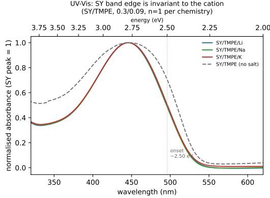
Figure 3.8: UV-Vis absorption of Super Yellow /TMPE blend films (lead composition 0.3/0.09; Au-electrode 2025 generation; one specimen per chemistry), normalised to the Super Yellow \pi - \pi^* peak. The peak ( \approx 446 nm) and the absorption onset ( \approx 2.50 eV) are superimposed for \text{Li}^+ , \text{Na}^+ , and \text{K}^+ ; the salt-free control (dashed) coincides at the band edge (its differing blue side and lower absolute absorbance are thickness/scattering, not electronic). The cation does not shift the semiconductor’s optical gap. Only band positions are read (absorbance magnitudes are thickness-confounded); analysis in scripts/ch3_uvvis.py , assessment in handouts/18_uvvis_assessment.md .
