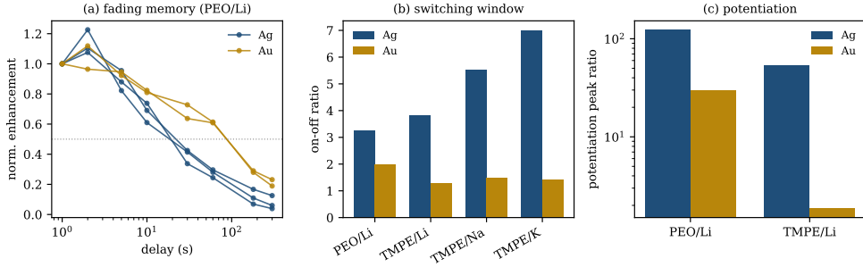
Figure 3.11: Illustrative electrode contrast at the lead composition (0.3/0.09). (a) Fading-memory decays of PEO/LiOTf devices, normalised to the first read: the gold curves (gold) cross half-enhancement later than the silver ones (blue), i.e. gold retains longer . (b) The steady-state switching window (on-off ratio) is narrower on gold for every chemistry, and is flat across the TMPE cation series on gold (no Li/Na/K ordering). (c) Pulse-potential dynamic range (peak ratio, log scale) is far smaller on gold. The inert electrode thus gives a weaker, higher-threshold, but more retentive response. Small n per cell, no human curve curvation on the gold side, and a generation offset between the corpora (see text); analysis in scripts/ch3_electrode.py , per-cell values in handouts/ch3_electrode_by_cell.csv .
