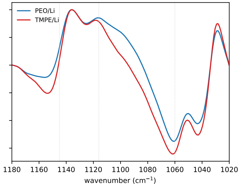
C-O-C envelope, powder repeat
