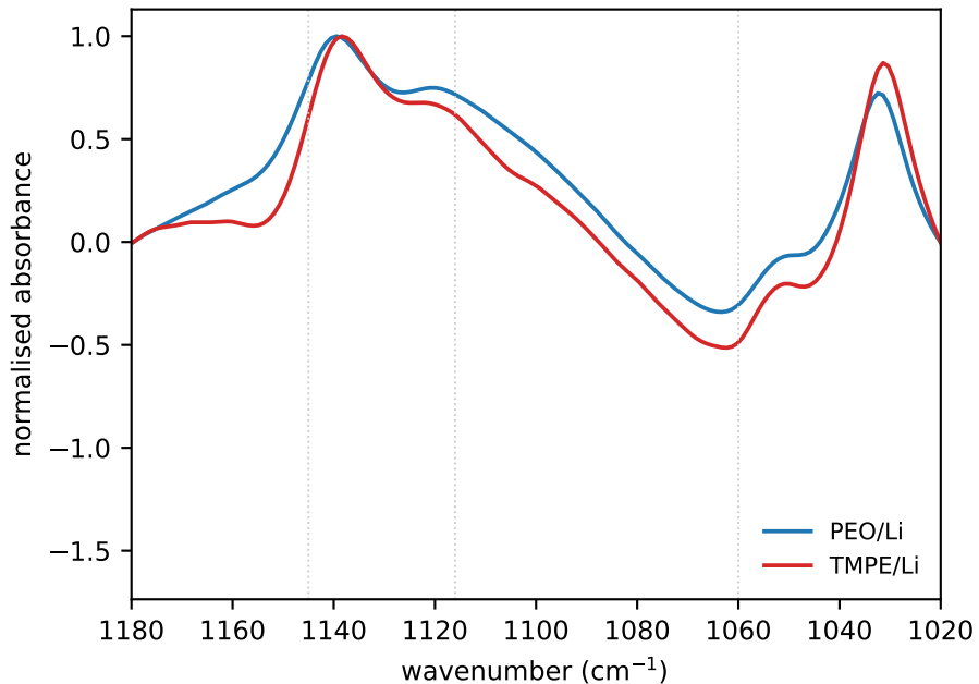
C-O-C envelope, film pair
