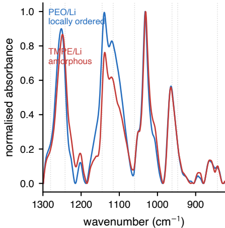
b host C–O–C order (Li, film)
