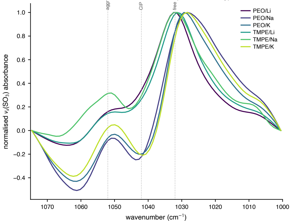
Triflate ion-association band ( n=1 / chemistry)
