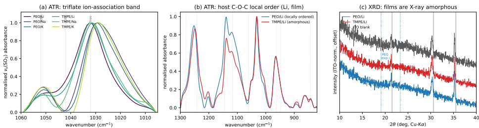
Figure 3.6: Microscopic corroboration of the chemistry axis (electrode-free Super Yellow -blend films/powders, 0.3/0.09, one specimen per chemistry). (a) ATR-FTIR triflate ion-association band \nu_s(\text{SO}_3) , whose position reports the ion-association state (spectroscopically free near 1032\text{ cm}^{-1} , contact ion pair near 1042\text{ cm}^{-1} , aggregate above; reference positions dotted [2]): it sits at 1029\text{ cm}^{-1} – 1032\text{ cm}^{-1} in every host \times cation sample with no cation-resolved shift — microscopically consistent with the cation not being a clean retention lever. (b) ATR-FTIR C–O–C envelope: the linear PEO host (blue) shows a resolved multiplet, i.e. retained local (conformational) ether-backbone order, whereas the hyperbranched TMPE host (red) collapses it into a single broad, amorphous band [2]. (c) X-ray diffraction of PEO/Li and TMPE/Li with a bare-ITO blank: all patterns show only the crystalline ITO substrate reflections (grey lines; 21.5^\circ , 30.6^\circ and 35.5^\circ ), with no sharp PEO crystalline doublet (blue dotted; 19.1^\circ and 23.3^\circ ) and no crystalline salt phase — the composite films are X-ray amorphous, so PEO’s order in (b) is short-range, not bulk crystallinity [2, 3]. ATR spectra normalised after a local/rubber-band baseline and XRD normalised to the ITO peak; intensities are not comparable across specimens (mixed film/powder sampling and thin films), so only band positions and shapes are read. Analysis in scripts/ch3_iratr.py and scripts/ch3_xrd.py ; assessments in handouts/16_iratr_assessment.md and 17_xrd_assessment.md .
