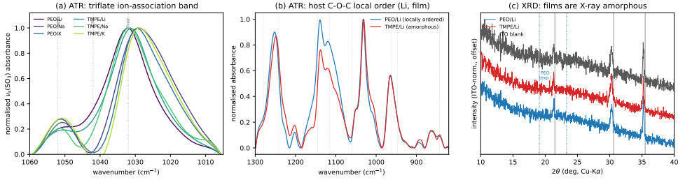
Figure 4.6: Microscopic corroboration of the chemistry axis (electrode-free Super Yellow -blend films/powders, 0.3/0.09, one specimen per chemistry). (a) ATR-FTIR triflate ion-association band \nu_s(\text{SO}_3) , whose position reports the ion-association state (spectroscopically free near 1032\text{ cm}^{-1} , contact ion pair near 1042\text{ cm}^{-1} , aggregate above; reference positions dotted [2]): it sits at 1029\text{ cm}^{-1} – 1032\text{ cm}^{-1} in every host \times cation sample with no cation-resolved shift — microscopically consistent with the cation not being a clean retention lever. (b) ATR-FTIR C–O–C envelope: the linear PEO host (blue) shows a resolved multiplet, i.e. retained local (conformational) ether-backbone order, whereas the hyperbranched TMPE host (red) collapses it into a single broad, amorphous band [2]. (c) X-ray diffraction of PEO/Li and TMPE/Li with a bare-ITO blank: all patterns show only the crystalline ITO substrate reflections (grey lines; 21.5^\circ , 30.6^\circ and 35.5^\circ ), with no sharp PEO crystalline doublet (blue dotted; 19.1^\circ and 23.3^\circ ) and no crystalline salt phase — the composite films are X-ray amorphous, so PEO’s order in (b) is short-range, not bulk crystallinity [2, 3]. ATR spectra normalised after a local/rubber-band baseline and XRD normalised to the ITO peak; intensities are not comparable across specimens (mixed film/powder sampling and thin films), so only band positions and shapes are read. Analysis in scripts/ch3_iratr.py and scripts/ch3_xrd.py ; assessments in handouts/16_iratr_assessment.md and 17_xrd_assessment.md .
