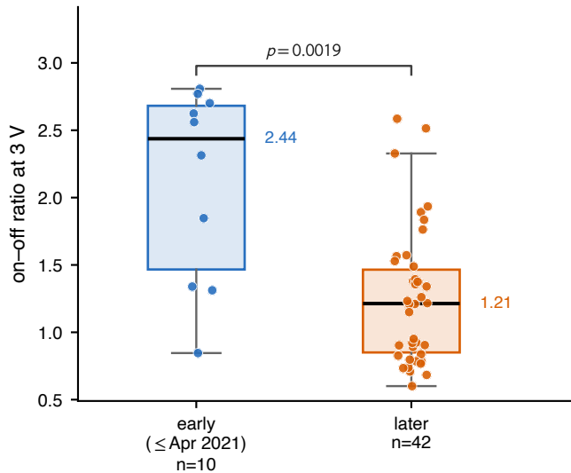
a switching window
