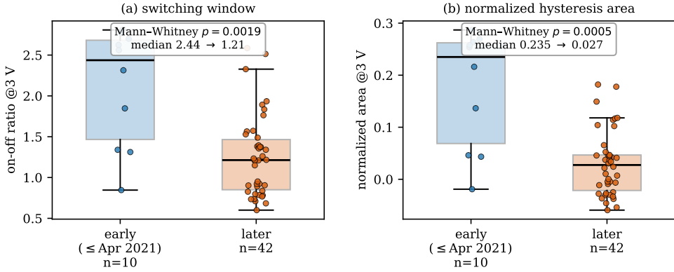
Figure 3.1: Switching-window collapse across the campaign on the standard Super Yellow/Hybrane/LiOTf/Ag corpus, read at the \sim 3 V stratum where the window is expressed, one value per device. (a) On–off ratio and (b) normalized hysteresis area, both for devices fabricated before the NM_v026 inflection ( \leq Apr 2021) versus later. Boxes are quartiles; points are individual devices; the annotated p is a two-sided Mann–Whitney test. The window collapses by roughly a factor of two in on–off ratio and an order of magnitude in area. Reproduced by scripts/bridge_figures.py (F1).
