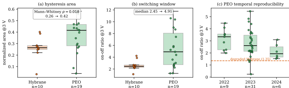
Figure 3.4: Resolution of the reproducibility crisis by switching to a PEO host (silver electrode, \sim 3 V, per device). (a) Normalized hysteresis area and (b) on-off ratio are larger for PEO than for contemporaneous Hybrane valid devices ( p = 0.018 for area). (c) PEO temporal reproducibility: the per-device on-off ratio holds at a usable level (median \approx 2.6 ) across 2022–2024 with no collapse, well above the degraded- Hybrane level (dashed line, 1.35). Reproduced by scripts/bridge_figures.py (F3).
