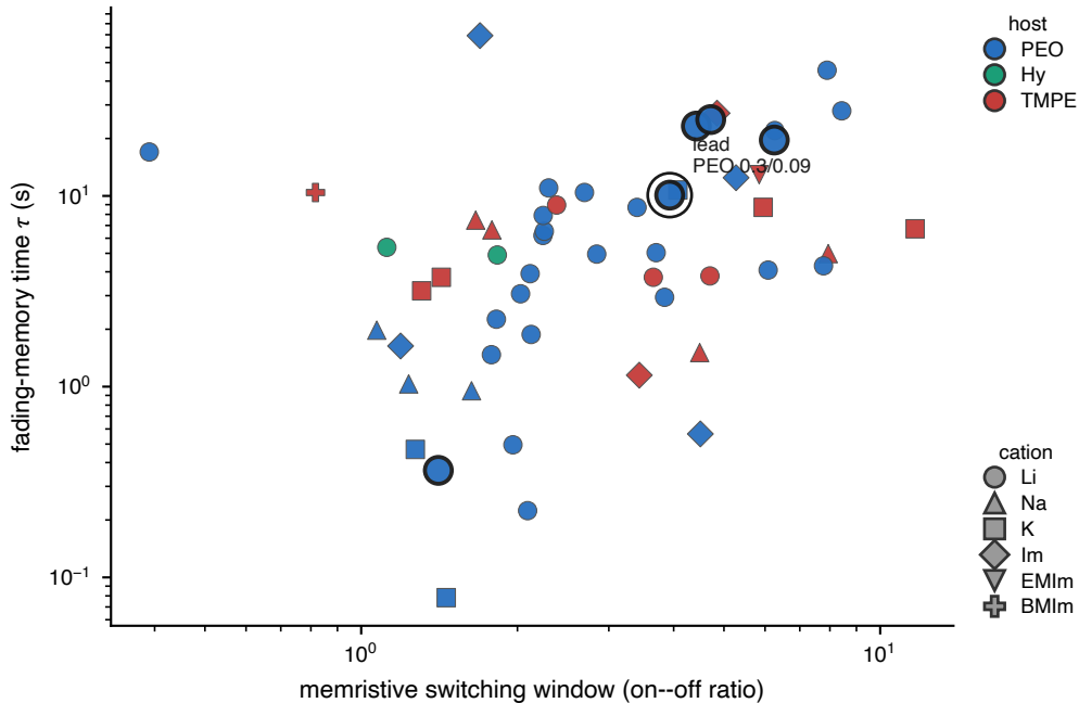
measured device palette (Ag, all chemistries; n=54 )
