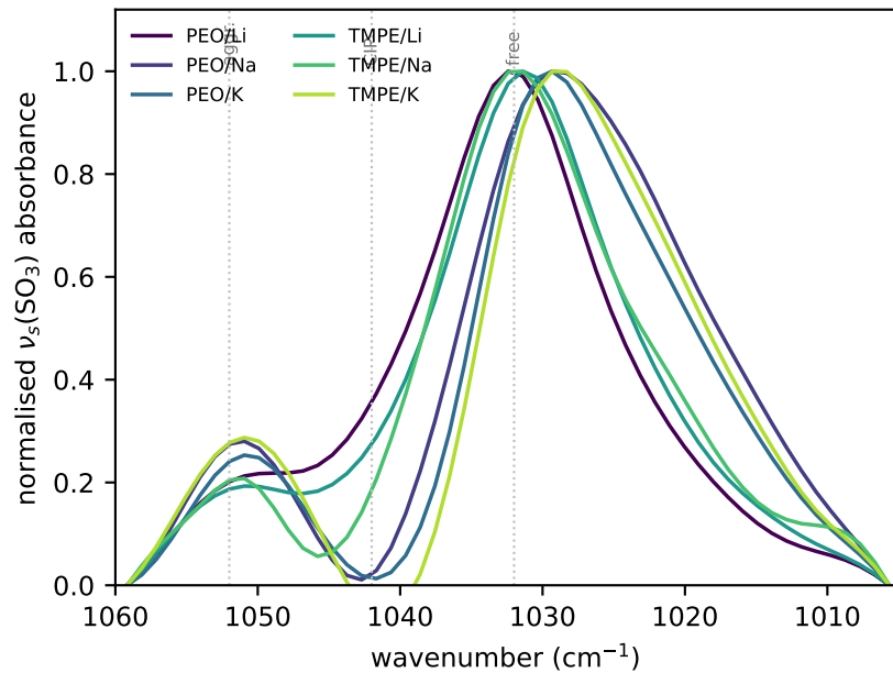
(a) ATR: triflate ion-association band
