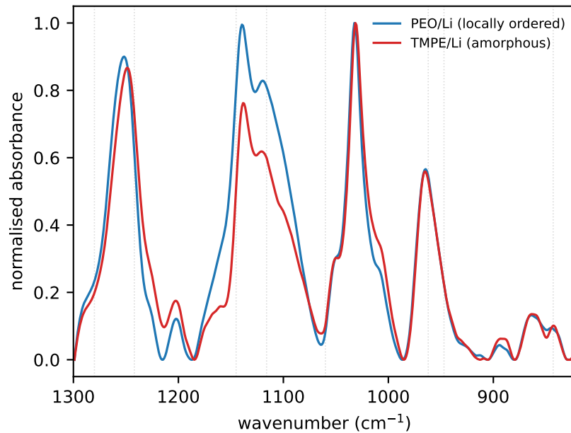
(b) ATR: host C-O-C local order (Li, film)
