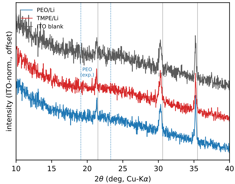
(c) XRD: films are X-ray amorphous
