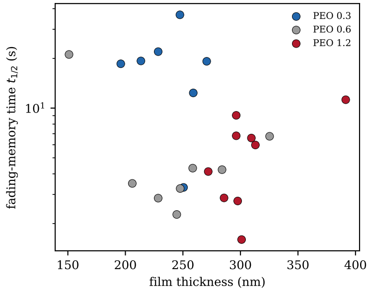
(b) memory tracks PEO, not thickness r(\text{thick}, t_{1/2} | \text{PEO}) = +0.05 (n=25)
