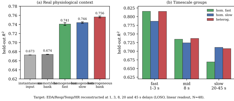
Figure 4.5: Multi-lag physiological context reconstruction on real WESAD streams (chest EDA, respiration, temperature, and ECG-derived heart rate). A linear read-out reconstructs each channel at delays of 1, 3, 8, 20 and 45s from the reservoir state (leave-one-subject-out, N = 48 ). The heterogeneous composition bank gives the best single-bank held-out R^2 (0.756) across the full fast-to-slow context vector, ahead of the best same-size homogeneous control (0.744) and well ahead of instantaneous input (0.673). Fast and slow homogeneous banks each win only their own band.
