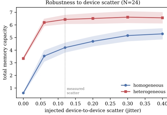
Figure 4.7: Total memory capacity versus the magnitude of injected device-to-device scatter (jitter on \tau , \beta and \alpha ), for the homogeneous and heterogeneous banks ( N = 24 , ten seeds; shaded bands \pm 1 SD). The heterogeneous bank keeps its advantage across the entire realistic spread (dotted line: the measured scatter). A bank of perfectly identical nodes (zero scatter) is nearly memory-less because matched nodes are redundant: in the reservoir setting, solution-processing scatter is a computational resource rather than a yield defect.
