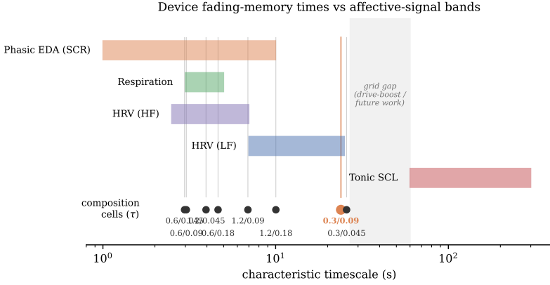
Figure 4.4: The Chapter 3-to-Chapter 4 bridge as a picture. Each PEO/LiOTf composition cell is placed at its measured fading-memory time \tau (markers, lower track) on the same logarithmic time axis as the characteristic timescale bands of the peripheral affective signals (coloured bars; table 4.1). The composition grid ( \tau \approx 3\text{--}26\text{ s} ) spans the phasic-EDA, respiration and HRV bands, with the lead cell PEO 0.3/0.09 (orange) sitting in the slow LF-HRV band. The tonic, minutes-scale band is not reached by composition alone (shaded gap) and would require the drive-amplitude knob of ?? or a slower future cell. This is the visual form of the design rule: an application selects a timescale, and performance follows from how well the device family covers it.
