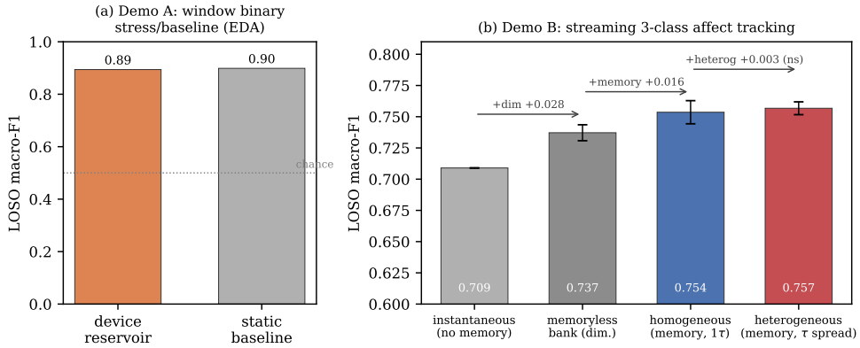
Figure 4.6: Affective computing with in-silico device reservoirs (leave-one-subject-out, linear read-out). (a) Demonstration A, window-level binary stress-versus-baseline from EDA: the single lead composition matches a static feature baseline, i.e. the 60 s-window task is quasi-static and requires no fading memory. (b) Demonstration B, streaming three-class affect tracking (baseline/stress/amusement) decomposed as instantaneous \rightarrow +dimensionality \rightarrow +fading memory \rightarrow +timescale heterogeneity. Fading memory contributes a small but consistent gain; the timescale-heterogeneity increment ( +0.005 \pm 0.011 ) is within seed noise. Error bars are \pm 1 SD over 10 bank seeds.
