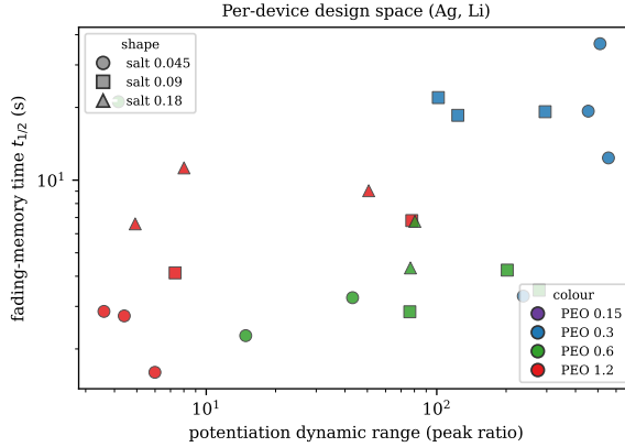
Figure 3.9: Per-device design space of the Super Yellow /PEO/LiOTf/Ag composition grid: fading-memory time t_{1/2} against potentiation dynamic range (peak ratio), coloured by PEO fraction and marked by salt fraction (one point per device, median over its pixels). The PEO fraction selects the broad region a device occupies — low PEO (blue) in the long-memory, high-dynamic-range corner, high PEO (red) in the opposite one, so memory and nonlinearity are not independently tunable but paired . The substantial within-composition scatter is the genuine device-to-device heterogeneity that Chapter 4 exploits; it is shown, not averaged away.
