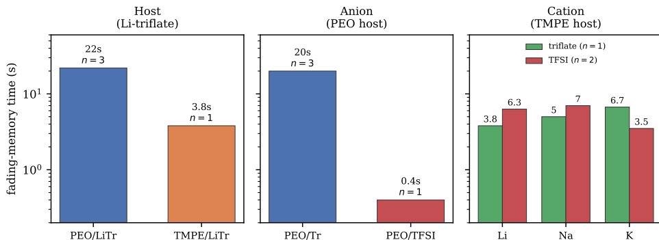
Figure 3.5: Illustrative effect of electrolyte chemistry on the fading-memory time constant ( Super Yellow , 0.3/0.09, silver, matched 4 V/2 V protocol). Host (PEO vs TMPE, Li-triflate) and anion (triflate vs TFSI, PEO host) produce the largest shifts. The cation panel shows the same three cations in the TMPE host under each anion: the order inverts with the anion (potassium longest in triflate, shortest in TFSI), so the cation produces no consistent, host- and anion-independent ordering. Sample sizes are small ( n as labelled); see text.
