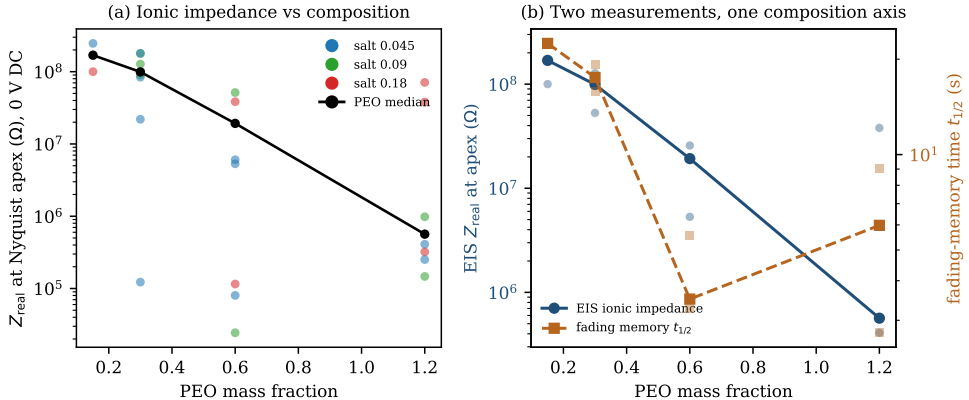
Figure 3.8: Equilibrium (0 V-DC) impedance spectroscopy corroborates the composition control of the dynamics (silver Super Yellow /PEO/LiOTf grid). (a) The impedance resistance scale — here the model-free real impedance at the Nyquist apex — falls by more than three orders of magnitude as the PEO fraction rises (points are devices, coloured by salt; the black line is the PEO median). (b) The equilibrium impedance scale (left axis) and the independently measured fading-memory time t_{1/2} (right axis) decline along the same PEO composition axis (cell-level points with per-PEO median trends): the two are co-driven by composition, not independent knobs. Analysis in scripts/ch3_eis.py ; per-cell values in handouts/ch3_eis_by_cell.csv .
