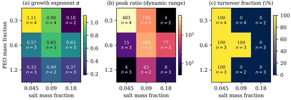
Figure 3.3: Potentiation (pulse-integration) response across the Super Yellow /PEO/LiOTf composition grid: (a) the log–log growth exponent \alpha , (b) the peak conductance ratio (usable dynamic range, log scale), and (c) the fraction of devices whose response turns over within the measured range ( N \leq 1000 ). Increasing the PEO fraction lowers \alpha and the dynamic range; increasing the salt fraction suppresses turnover, sustaining growth to higher pulse counts. Per-cell median, with the device count n annotated in each cell.
