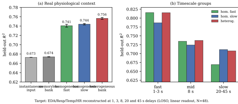
Figure 4.3: Multi-lag physiological context reconstruction on real WESAD streams (chest EDA, respiration, temperature, and ECG-derived heart rate). A linear read-out reconstructs each channel at delays of 1, 3, 8, 20 and 45 s from the reservoir state (leave-one-subject-out, N = 48 ). The heterogeneous composition bank gives the best single-bank held-out R^2 (0.756) across the full fast-to-slow context vector, ahead of the best same-size homogeneous control (0.744) and well ahead of instantaneous input (0.673). Fast and slow homogeneous banks each win only their own band.
