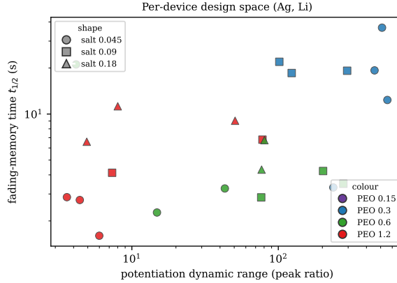
Figure 3.10: Per-device design space of the Super Yellow /PEO/LiOTf/Ag composition grid: fading-memory time t_{1/2} against potentiation dynamic range (peak ratio), coloured by PEO fraction and marked by salt fraction (one point per device, median over its pixels). The PEO fraction selects the broad region a device occupies — low PEO (blue) in the long-memory, high-dynamic-range corner, high PEO (red) in the opposite one, so memory and nonlinearity are not independently tunable but paired . The substantial within-composition scatter is the genuine device-to-device heterogeneity that Chapter 4 exploits; it is shown, not averaged away.
