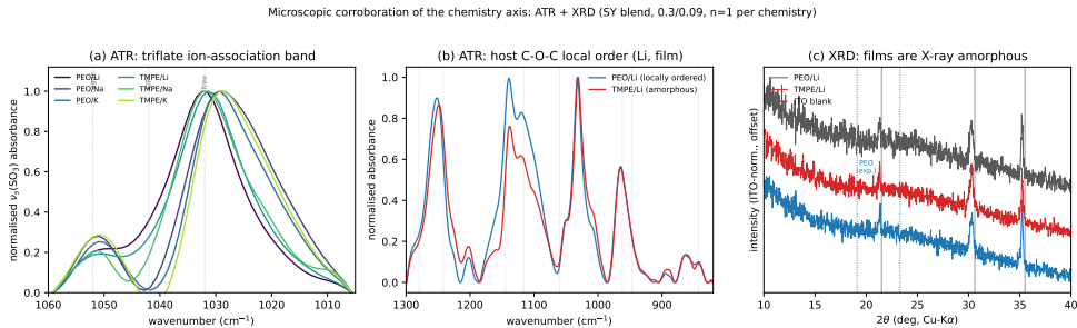
Figure 3.4: Microscopic corroboration of the chemistry axis (electrode-free Super Yellow -blend films/powders, 0.3/0.09, one specimen per chemistry). (a) ATR-FTIR triflate ion-association band \nu_s(\text{SO}_3) , whose position reports the ion-association state (spectroscopically free near 1032\text{ cm}^{-1} , contact ion pair near 1042\text{ cm}^{-1} , aggregate above; reference positions dotted): it sits at 1029\text{ cm}^{-1} – 1032\text{ cm}^{-1} in every host \times cation sample with no cation-resolved shift — microscopically consistent with the cation not being a clean retention lever. (b) ATR-FTIR C–O–C envelope: the linear PEO host (blue) shows a resolved multiplet, i.e. retained local (conformational) ether-backbone order, whereas the hyperbranched TMPE host (red) collapses it into a single broad, amorphous band. (c) X-ray diffraction of PEO/Li and TMPE/Li with a bare-ITO blank: all patterns show only the crystalline ITO substrate reflections (grey lines; 21.5^\circ , 30.6^\circ and 35.5^\circ ), with no sharp PEO crystalline doublet (blue dotted; 19.1^\circ and 23.3^\circ ) and no crystalline salt phase — the composite films are X-ray amorphous, so PEO’s order in (b) is short-range, not bulk crystallinity. ATR spectra normalised after a local/rubber-band baseline and XRD normalised to the ITO peak; intensities are not comparable across specimens (mixed film/powder sampling and thin films), so only band positions and shapes are read. Analysis in scripts/ch3_iratr.py and scripts/ch3_xrd.py ; assessments in handouts/16_iratr_assessment.md and 17_xrd_assessment.md .
