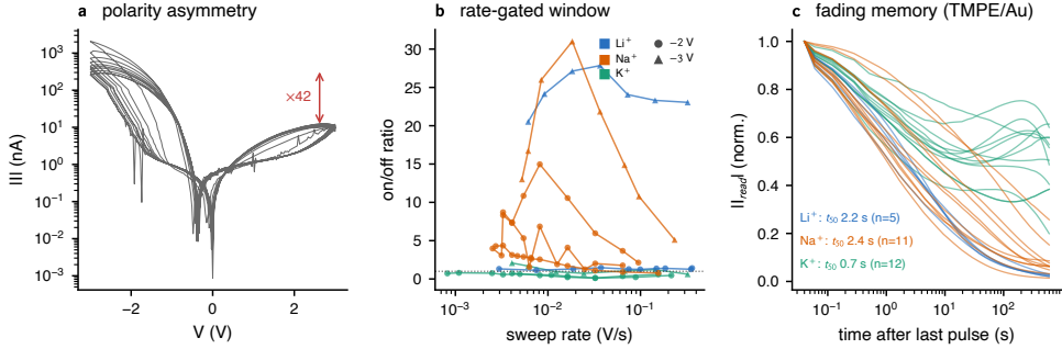
Figure 4.12: The negative-polarity face of the gold/TMPE/triflate devices (illustrative tier; section C.7). (a) Exemplar bipolar sweep ( \pm 3 V, ten cycles, Na + device): the negative branch carries \approx 42\times the current of the positive one. (b) The switching window is rate-gated: on–off ratio against sweep rate for all step-count series (colour = cation, marker = amplitude); slow sweeps open windows of 20–31 where the standard fast protocol reads \approx 1 . (c) Fading memory of the TMPE host on gold: sparse-read relaxations after -5 V pulse trains, normalised to the first read, with per-cation median half-decay times, seconds-scale, as on silver, and far below PEO on gold.
