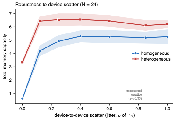
Figure 5.9: Total memory capacity versus the magnitude of injected device-to-device scatter (jitter on \tau , \beta and \alpha ), for the homogeneous and heterogeneous banks ( N = 24 , ten seeds; shaded bands \pm 1 SD). The heterogeneous bank keeps its advantage across the entire realistic spread, including at the measured device-to-device scatter (dotted line: \sigma(\ln \tau) \approx 0.85 , derived in section D.3). A bank of perfectly identical nodes (zero scatter) is nearly memory-less because matched nodes are redundant: the scatter that yield engineering fights to remove is what the reservoir computes on.
