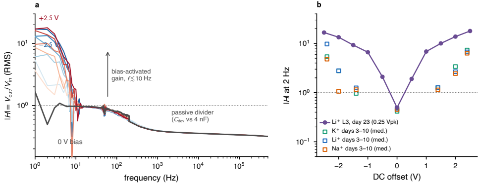
Figure 4.13: Frequency-domain face of the gold/TMPE/triflate devices (illustrative tier; section C.8). (a) Transfer ratio |H|(f) of one \text{Li}^+ junction in series with 4 nF (day 23, 0.25 Vpk) at eleven DC offsets from 0 (grey) to \pm 2.5 V (blue negative, red positive): above \sim 1 kHz all curves collapse onto the passive capacitive divider; below \sim 10 Hz the bias activates a fundamental-frequency gain of up to \approx 18 , monotone in bias magnitude and near-symmetric in its sign. (b) Bias-gain curve: |H| at 2 Hz against DC offset for the day-23 series (line) and the per-cation medians of the earlier sessions (squares; days 3–10, 0.4 Vpk–1.4 Vpk); gain requires bias, grows with it, and appears for all three cations.
