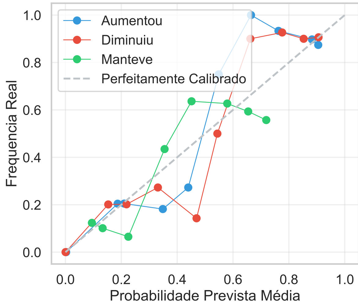
Reliability Diagram (Calibracao)
