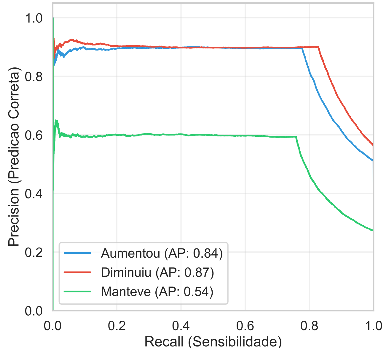
Precision-Recall Curve (OVR) no TESTE
