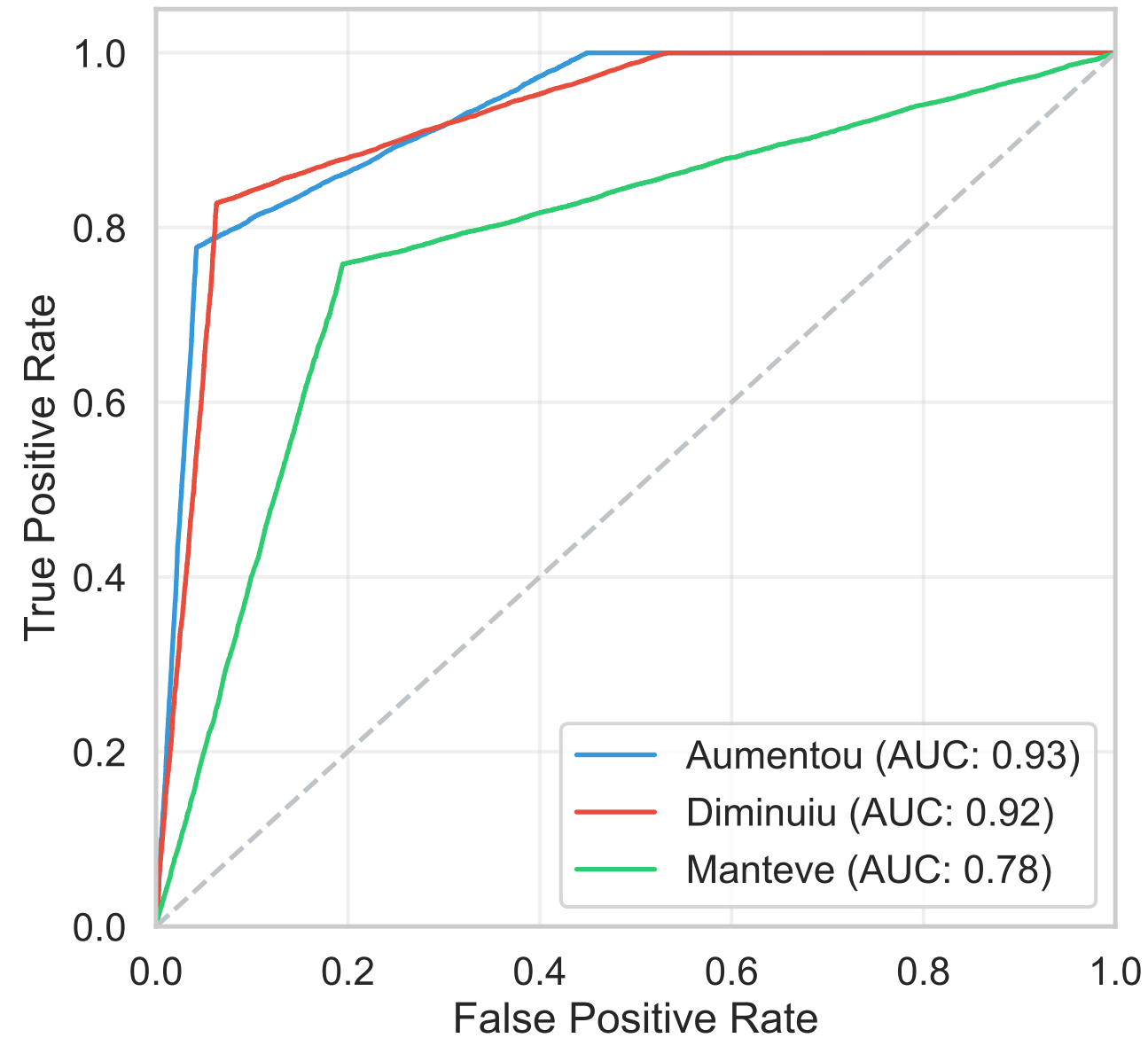
ROC Curve (One-vs-Rest) no TESTE
