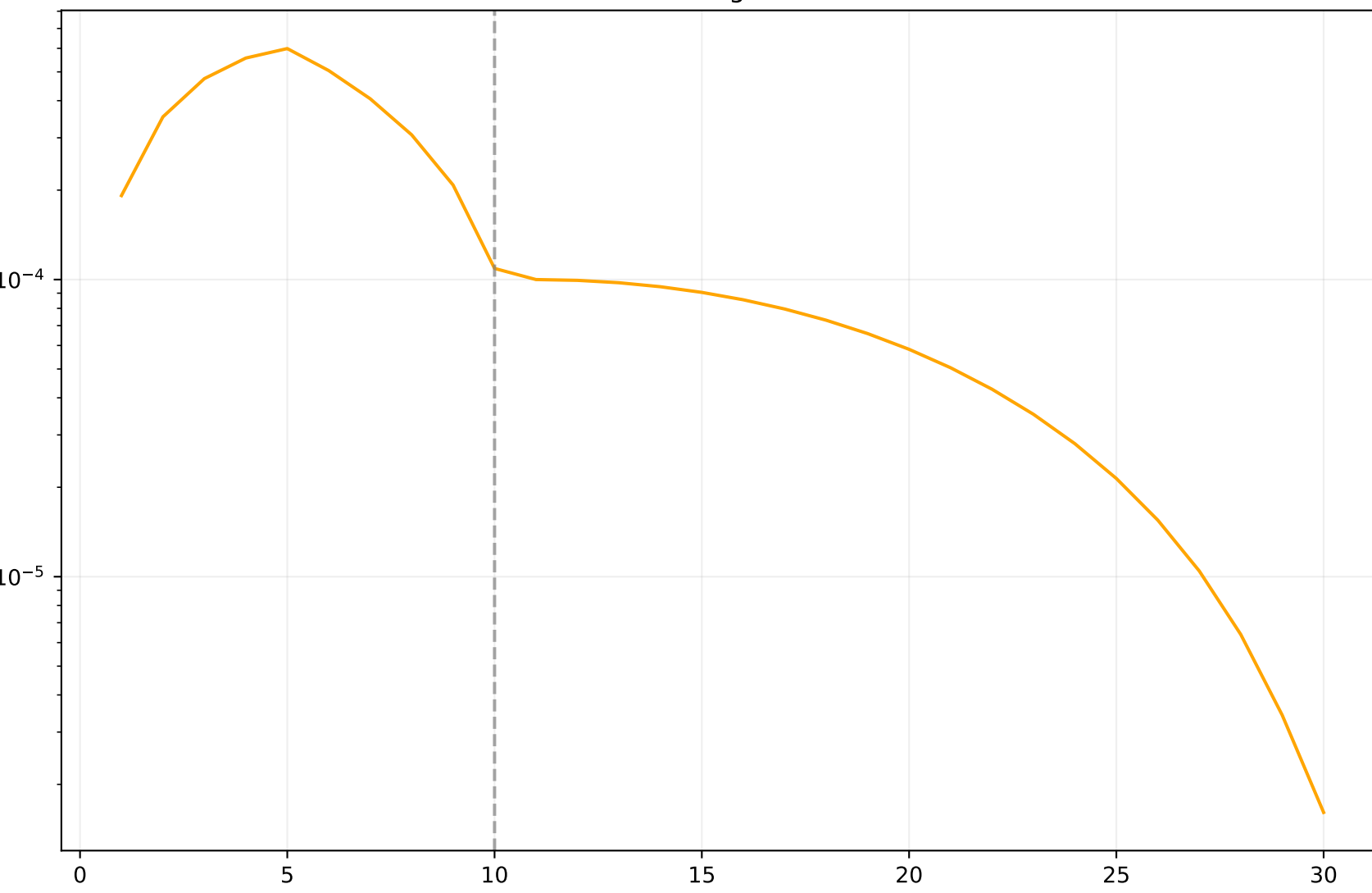
Learning Rate
