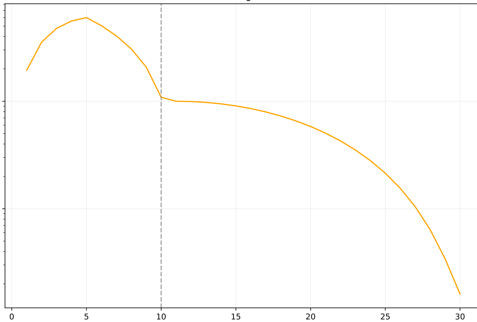
Learning Rate
