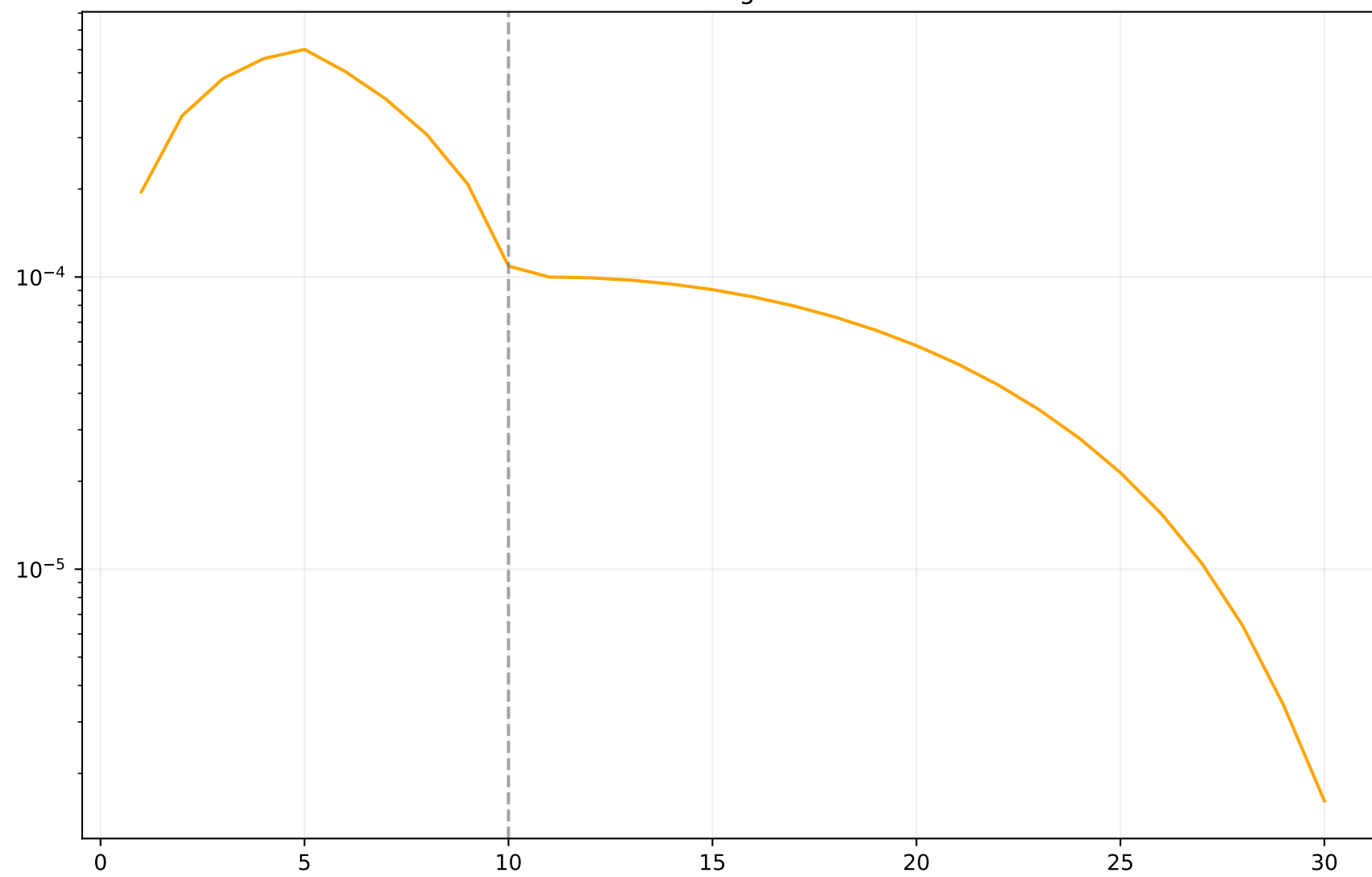
Learning Rate
