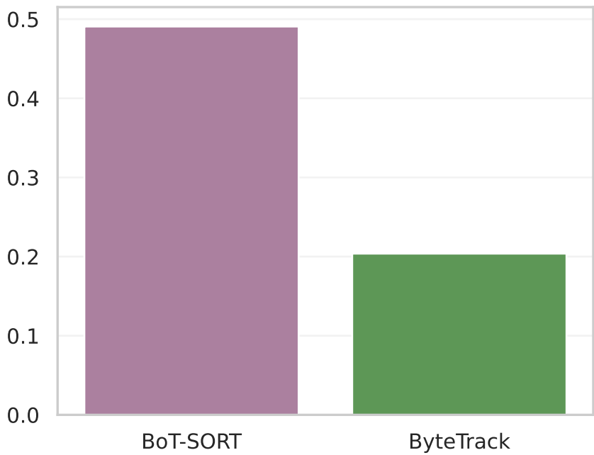
MOTP ↓
