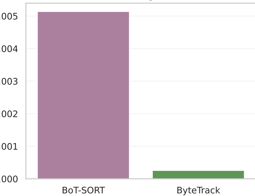
MT/obj ↑
