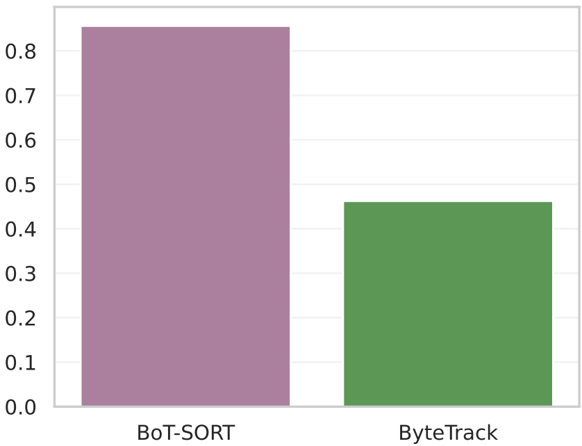
MOTA ↑
