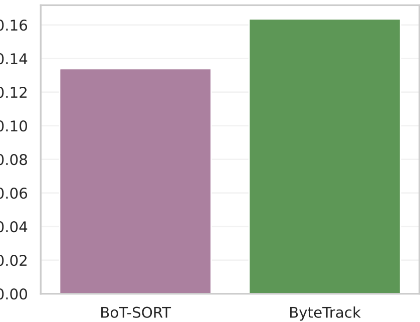
IDs/obj ↓
