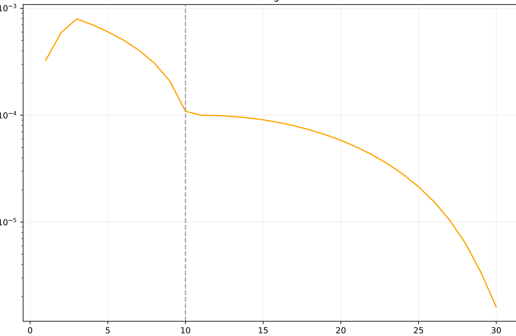
Learning Rate
