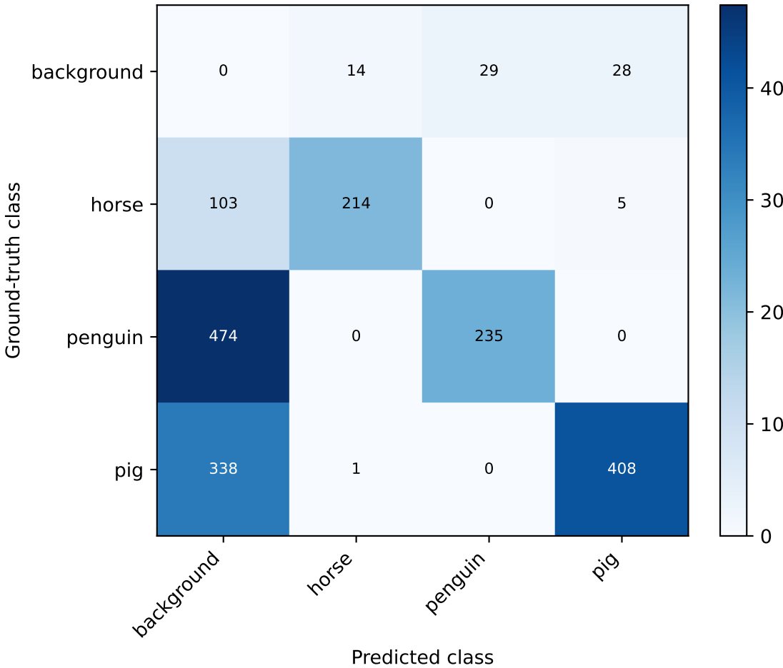
Confusion Matrix (Test)
