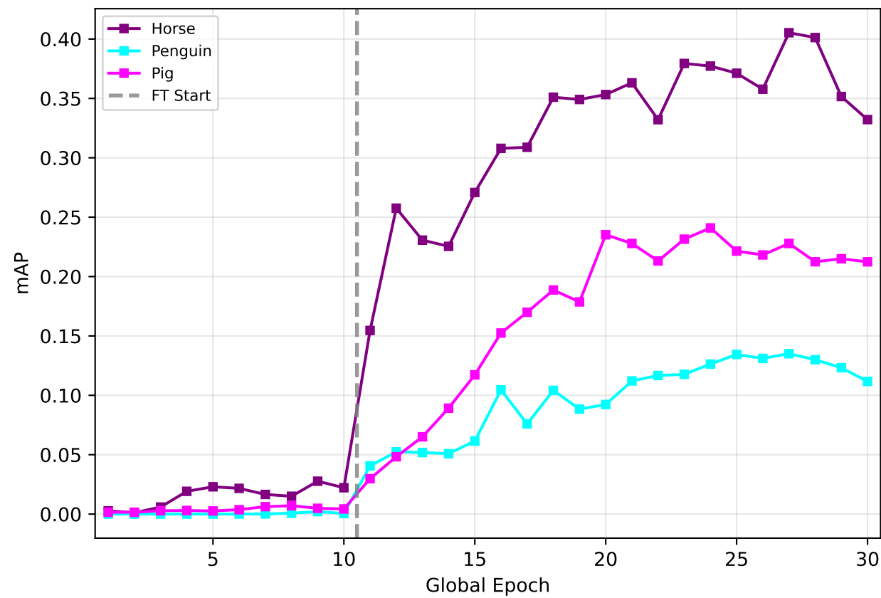
Per-Class mAP
