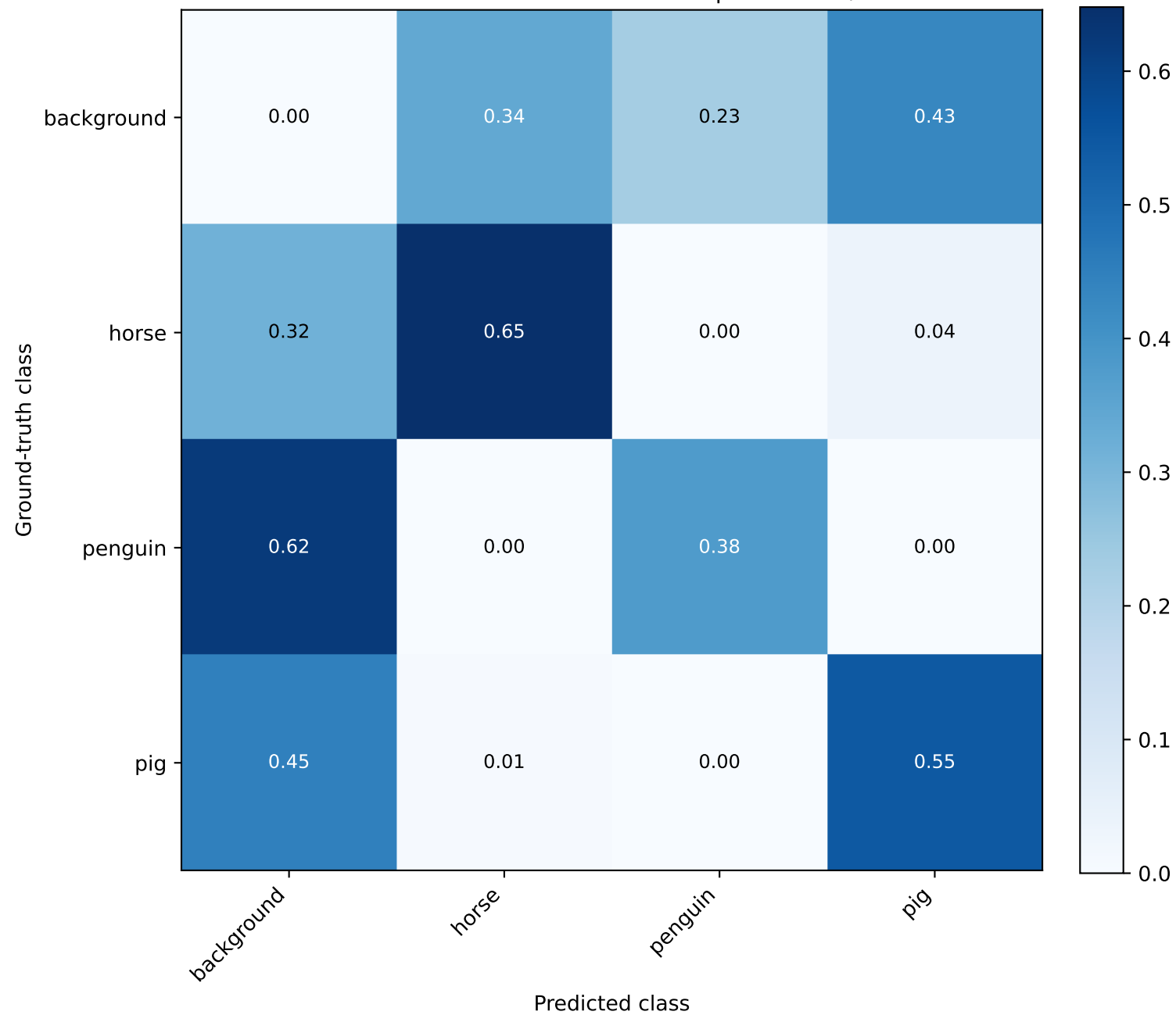
Normalized Detection Confusion Matrix | IoU=0.50, score=0.50
