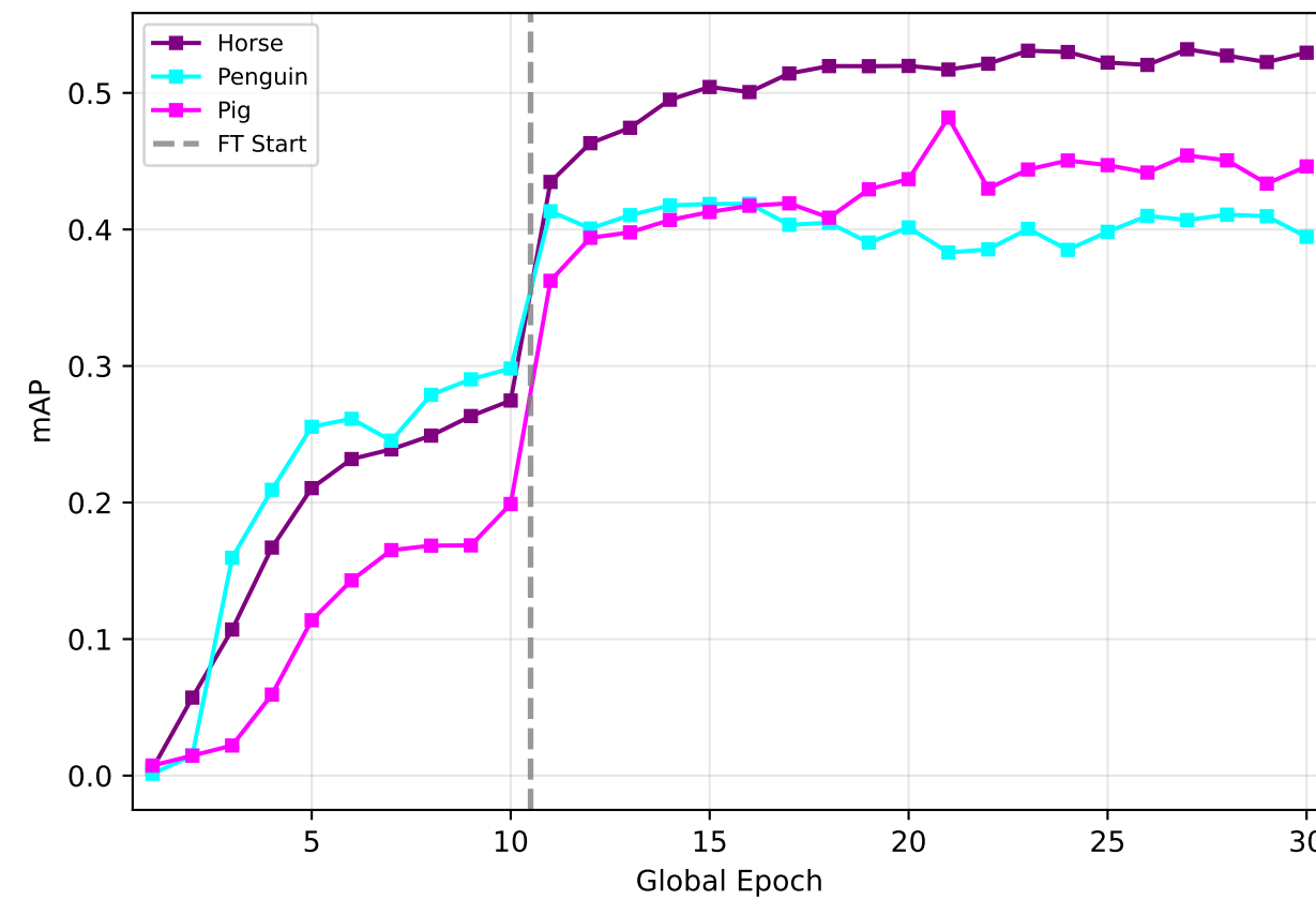
Per-Class mAP
