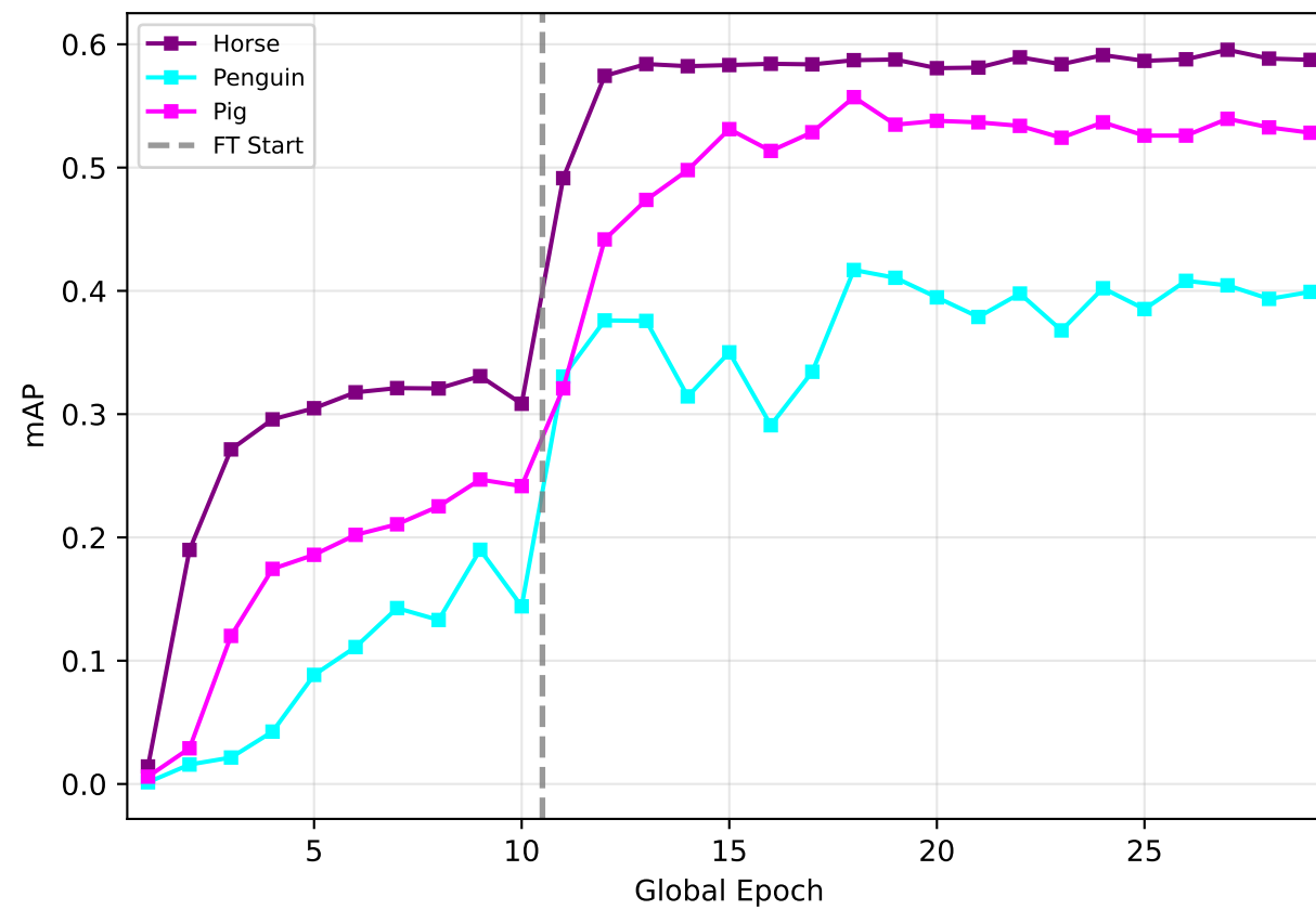
Per-Class mAP
