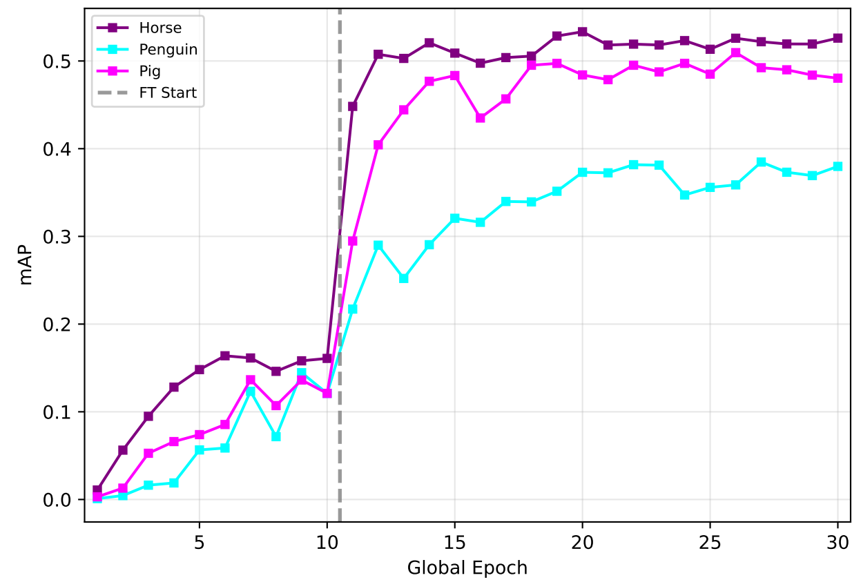
Per-Class mAP
